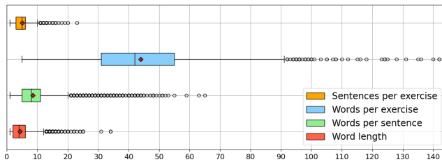
Figure 3: Exercise, sentence and word length distribution on the whole dataset.
