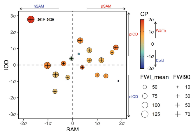
Fig. 4. Scatter plot of cumulative monthly fire weather indices FWI_mean and FWI90 in September–February in forested areas of NSW for the past 20 years (2001–2020) against the SAM, IOD, and central Pacific El Niño (CP). The three climate drivers are shown as cumulative values from September to February and are all normalized. The Indian Ocean Dipole (IOD) is measured by the Dipole Mode Index, SAM is an observation-based Southern Hemisphere Annular Mode Index, and CP is the central Pacific El Niño transformed by Niño4 and Niño3 indices [47].
