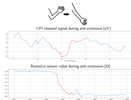
Figure 8: Arm extension illustration, with signal illustration from CP1, along with sensor variation.
