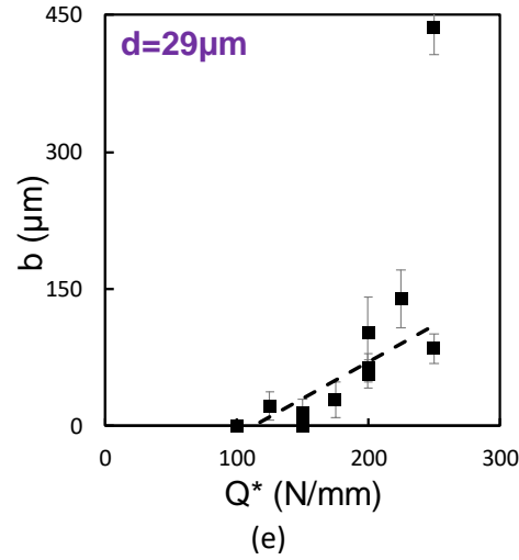
Figure 11: Projected crack length as a function of tangential load amplitude for different grain sizes of the C35 steel: : (a) d=3\mu\text{m} ; (b) d=6\mu\text{m} ; (c) d=12\mu\text{m} ; (e) d=20\mu\text{m} ; (e) d=29\mu\text{m} ( Q^* : tangential force amplitude; b : projected crack length).
