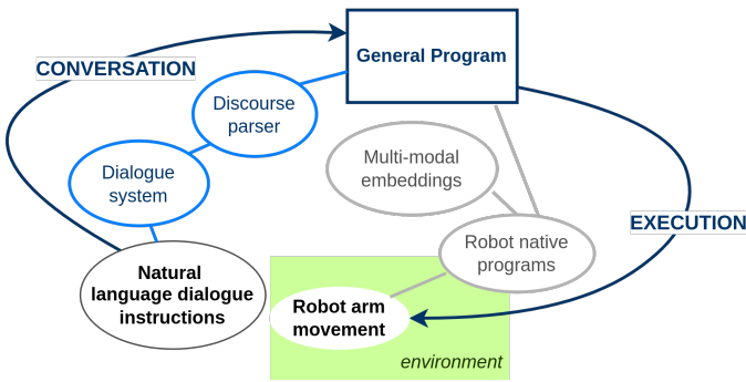
Figure 2. A schematic overview of the proposed system. The conversational dialogue leads to the construction of the general program, which can then be executed by a secondary program in varying environments.
