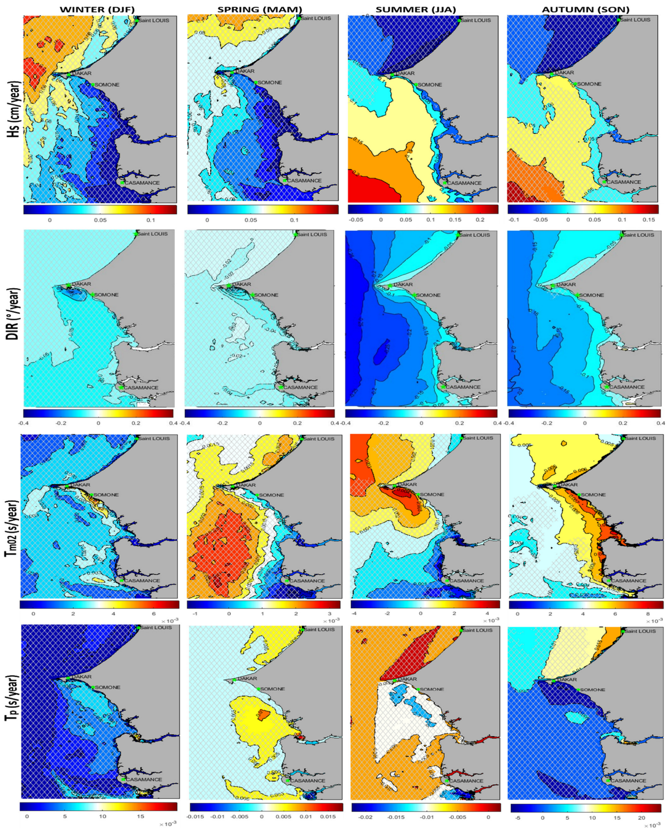
Figure 7. Seasonal trends computed over the period 1980–2021 for the main wave parameters (Hs, DIR, T_{m02} , and T_p ) in winter, spring, summer, and autumn on the Senegalese Coast from 1980–2021, Hatched zones on maps indicate areas where trends are not significant at 95% (Mann–Kendall test).
