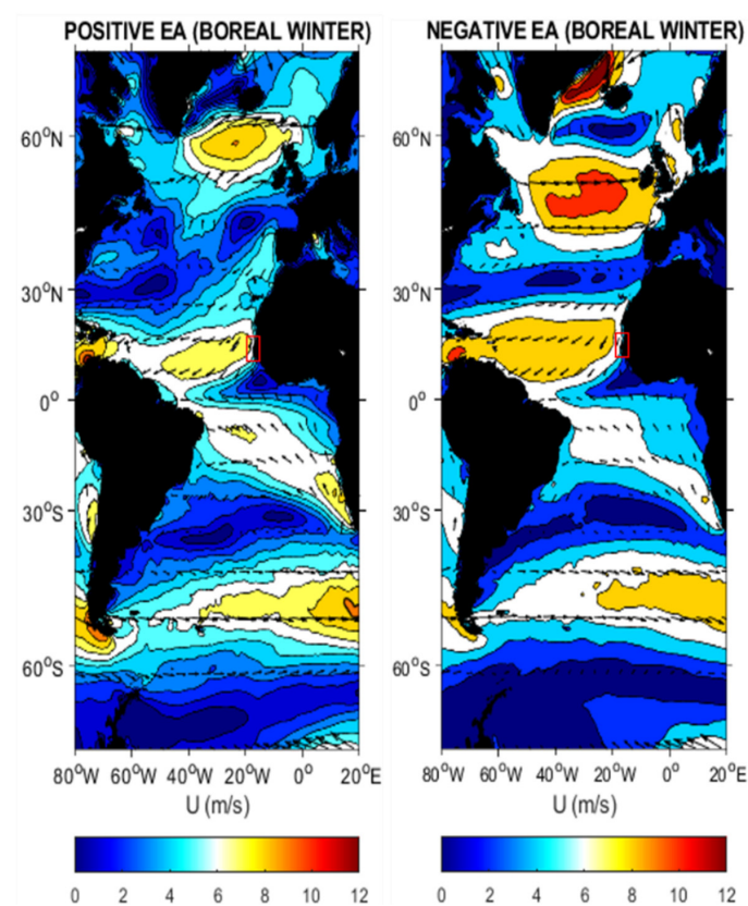
Figure 11. The red rectangle indicates the average winter wind speed corresponding, respectively, to the periods of maximum (EA+, left ) and minimum (EA−, right ) phases of EA mode in the tropical Atlantic on the Senegalese Coast.
