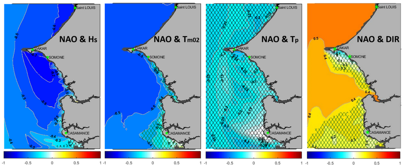
Figure 8. Spatial correlations between NAO and wave parameters ( H_s , T_{m02} , T_p , and DIR ) during boreal winter (DJFM), computed on the Senegalese Coast from 1980–2021, crosslines on maps indicate areas with non-significant correlations (at 95% confidence interval from Mann–Kendall test).
