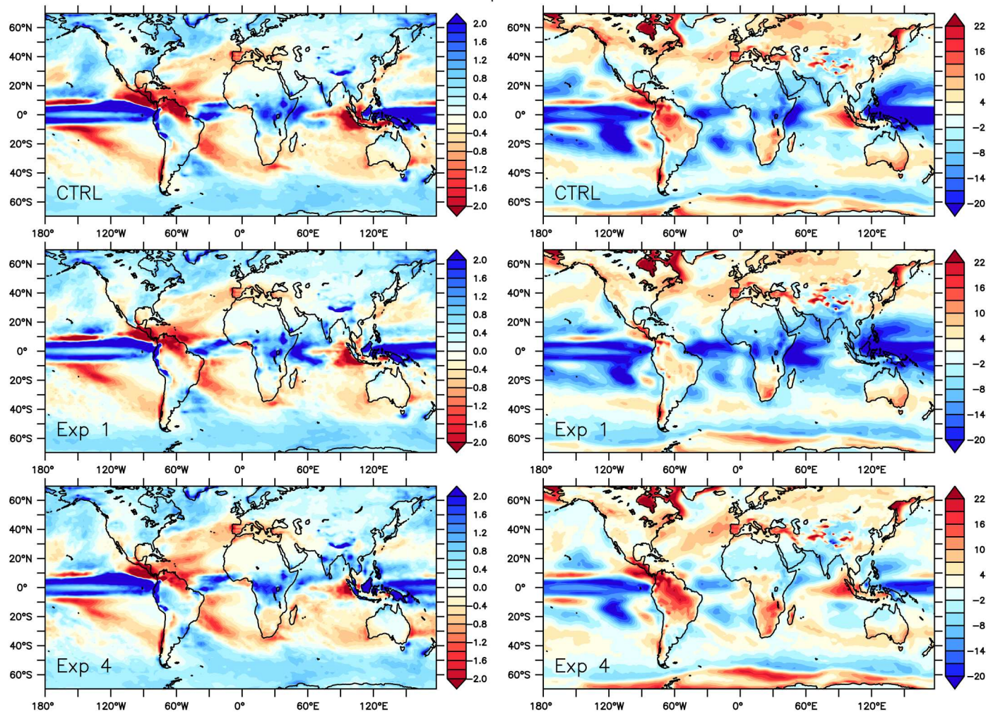
Fig. 5. Surface evaporation ( \text{mm}/\text{day} ) and surface net solar radiation change ( \text{W}/\text{m}^2 ) in coupled simulations for a global temperature change of 5.5 K. The maps correspond to differences between the abrupt4 \times\text{CO}_2 and piControl simulations, averaged over 21 consecutive years centered at year 33 for CTRL, year 65 for Exp 1, and year 17 for Exp 4.
