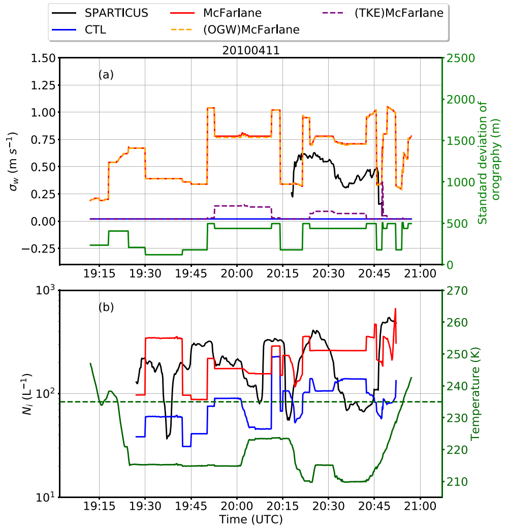
Figure 8. \sigma_w , N_i , and standard deviation of orography along the flight tracks on 11 April. The black lines are from observation, the blue lines are from the CTL simulation, and the red lines are from the modified model with the McFarlane scheme OGW-induced \sigma_w . The orange lines in (a) are the OGW component of simulated \sigma_w , and the pink lines are the CLUBB-TKE component of simulated \sigma_w . The green lines in (a) are the standard deviation of orography extracted from the model. The dark green solid lines in (b) are temperatures in the nudged McFarlane simulation. The dark green dashed lines in (b) are 235 K lines. The first and last 15 min of N_i during the flights are excluded to avoid bias due to the limitation of instruments when taking off and landing.
