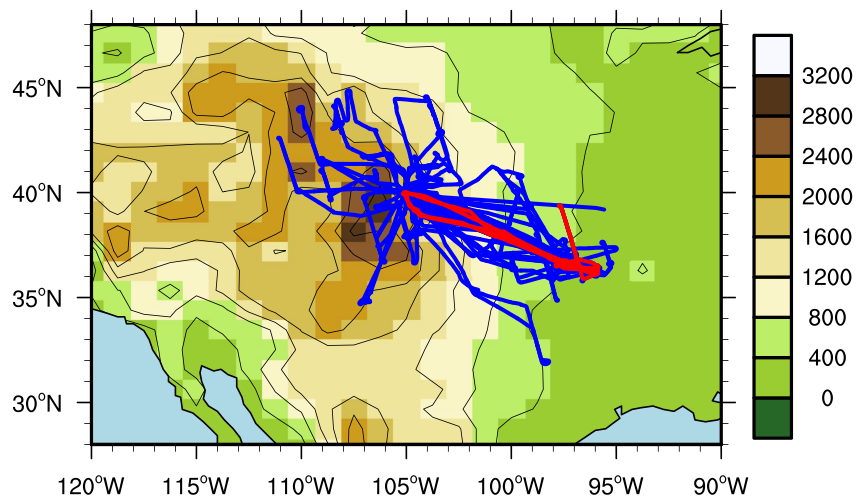
Figure 1. Aircraft trajectories (solid blue lines) during the SPARTICUS campaign. Color shading and black line contours show the surface terrain (unit: m). The solid red lines are flight tracks in the days (19, 30 March; 1, 28, and 29 April 2010) when ridge-crest cirrus was observed.
