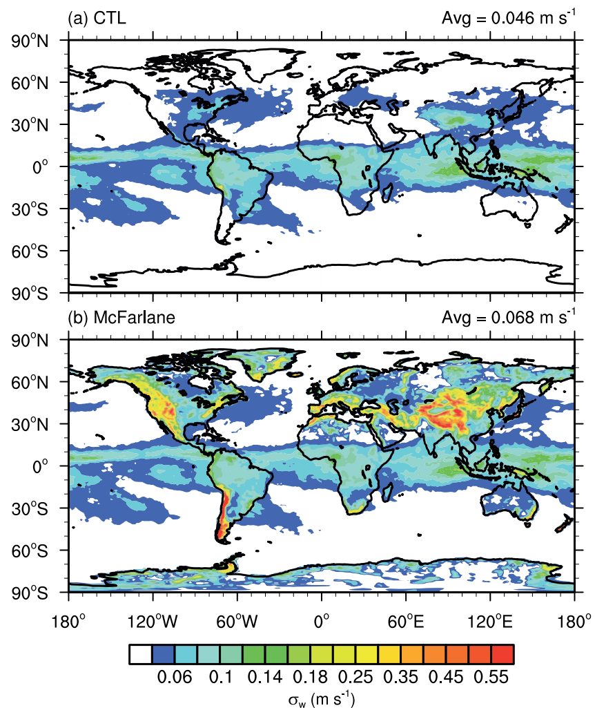
Figure 2. Global distribution of annual mean sub-grid scale vertical velocity variance ( \sigma_w ) for cirrus formation ( \text{m s}^{-1} ) from nudged simulations (a) CTL and (b) McFarlane during the SPARTICUS campaign in the upper troposphere (250 hPa). The value to the right of each title represents the global average weighted by the area.
