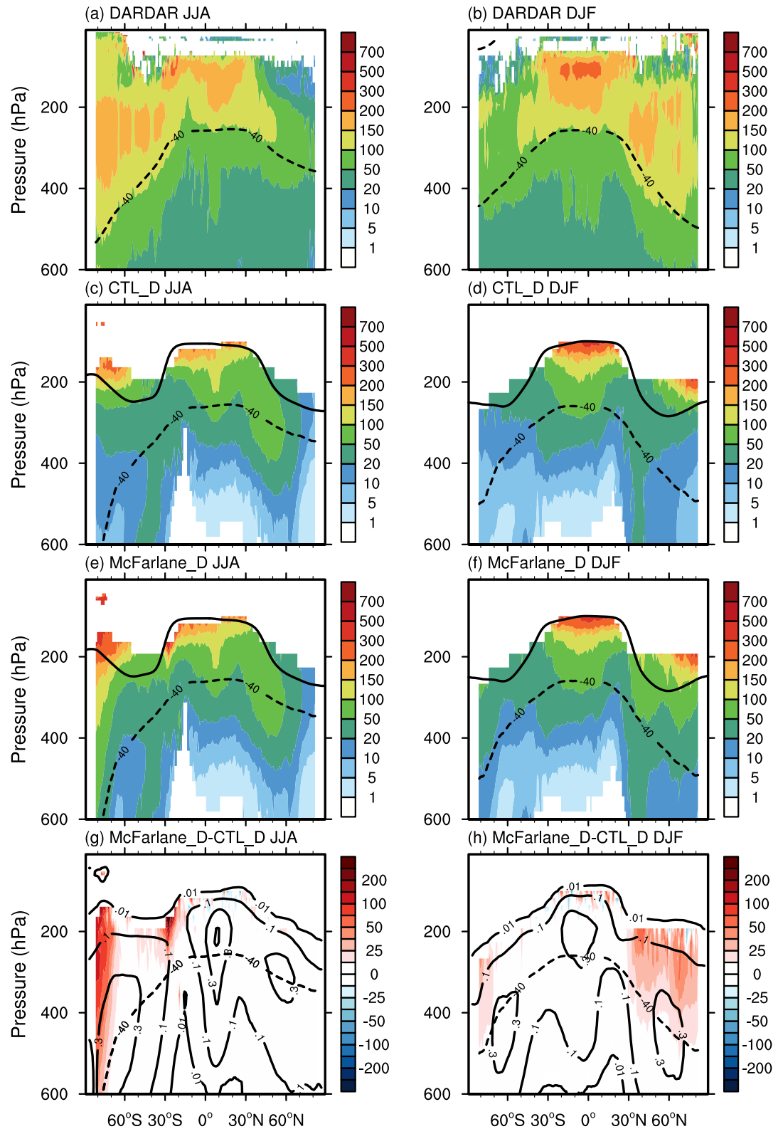
Figure 11. Seasonal zonal mean N_i between DARDAR and simulations (CTL_D and McFarlane_D) from 2007 to 2009 along the CALIPSO satellite tracks. The dashed line is the annual mean -40^{\circ}\text{C} isothermal line. The solid lines in (c), (d), (e), and (f) are the tropopause in the simulations. The solid lines in (g) and (h) are ice cloud frequencies in the McFarlane_D simulation. The N_i values are averaged over cloudy and clear-sky periods. Only N_i with diameters larger than 5\ \mu\text{m} , IWC \geq 1 \times 10^{-3}\ \text{g kg}^{-1} and grid ice cloud fraction larger than 0.01 are considered.
