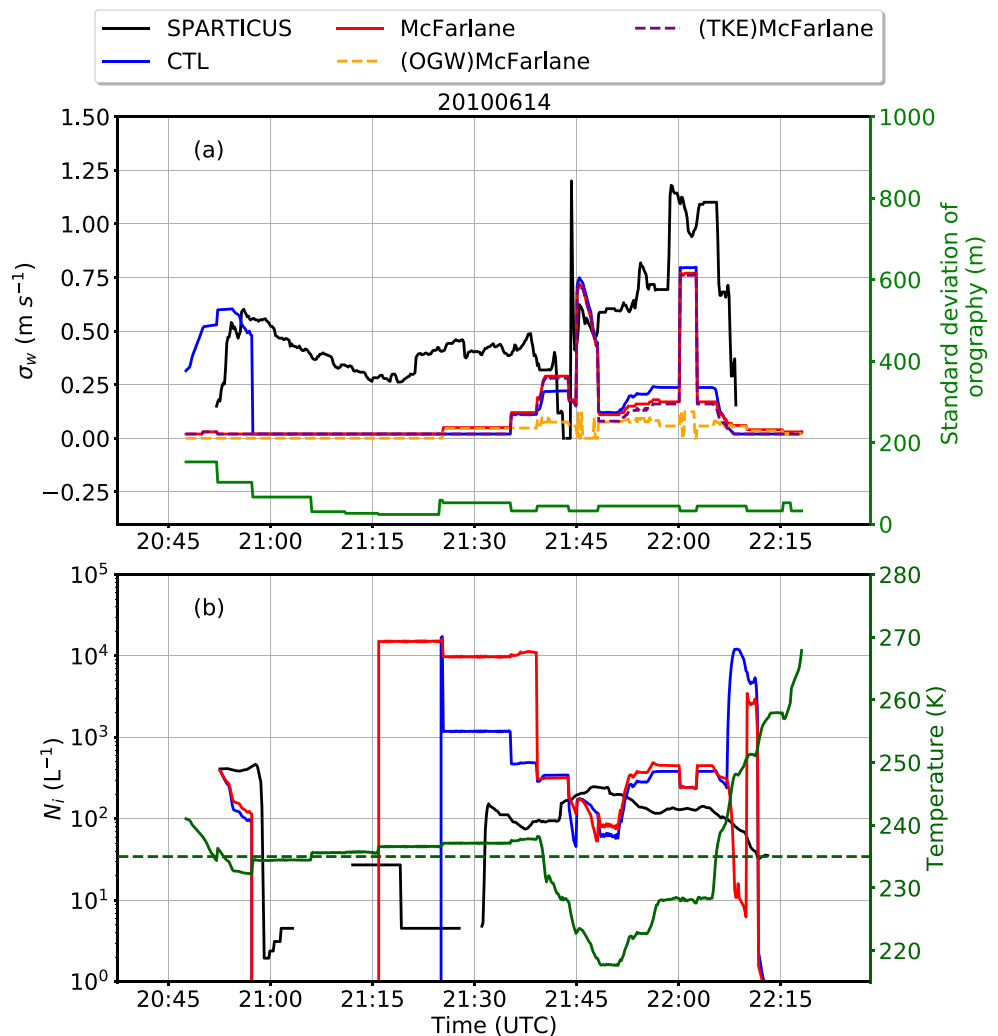
Figure 9. Similar to Figure 8 but along the flight tracks on 14 June 2010.
