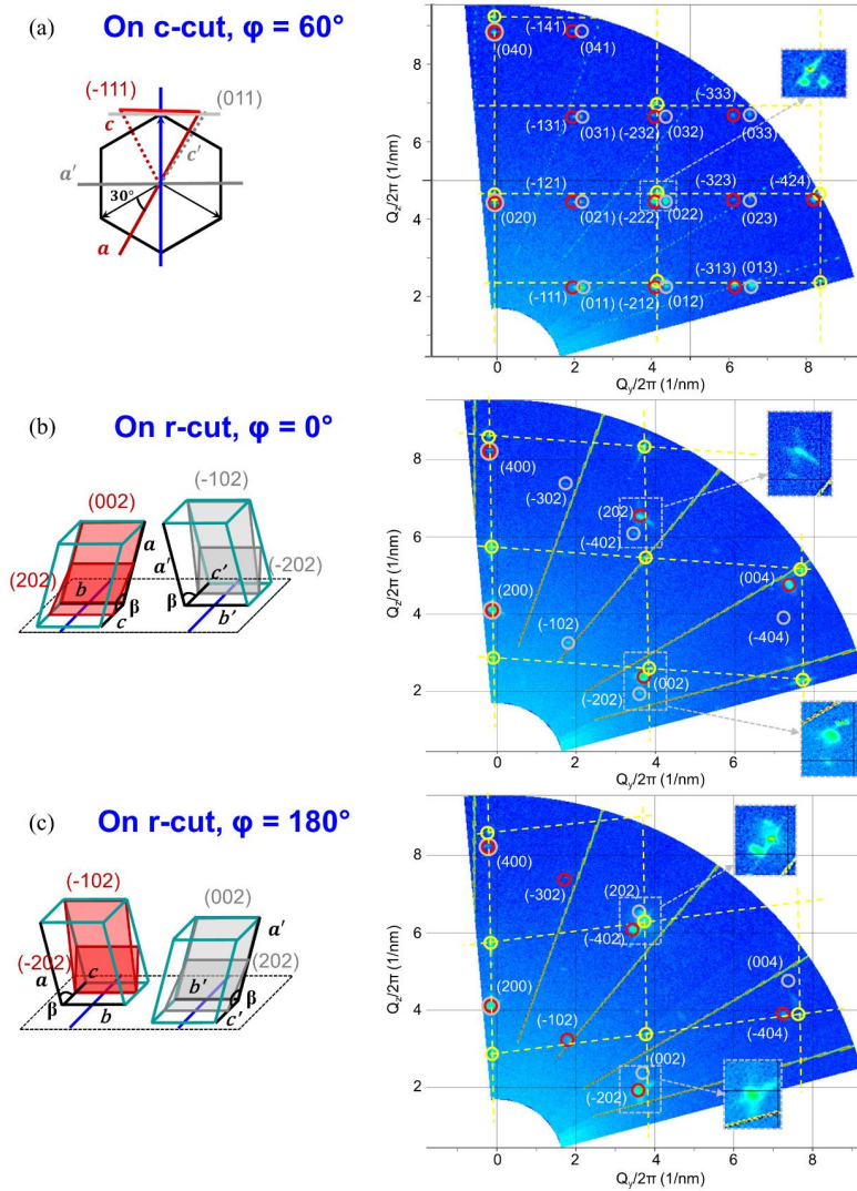
FIG. 3. Reciprocal space maps (RSM) of \text{VO}_2(\text{M1}) deposited on (a) c-cut sapphire substrate, taken along a_{\text{Al}_2\text{O}_3} azimuth, and (b, c) on r-cut sapphire, taken perpendicular to a_{\text{Al}_2\text{O}_3} azimuth with (b) along [1\bar{1}01] and (c) along [\bar{1}101] . The directions of the RSM scans are shown as blue lines on the unit cell sketches on the left of each map. The substrate peaks and reciprocal space lattice are shown in yellow. The \text{VO}_2(\text{M1}) peaks are indexed in white and circled in red or grey to differentiate between the two variants seen on each map. These variants are depicted on the left in corresponding colors (red and grey), with a few selected planes as example, to be related to the peaks seen on the maps. Close-up views of some areas of the RSM are also shown, to underline the 2 \text{VO}_2(\text{M1}) variants detected on each map.
