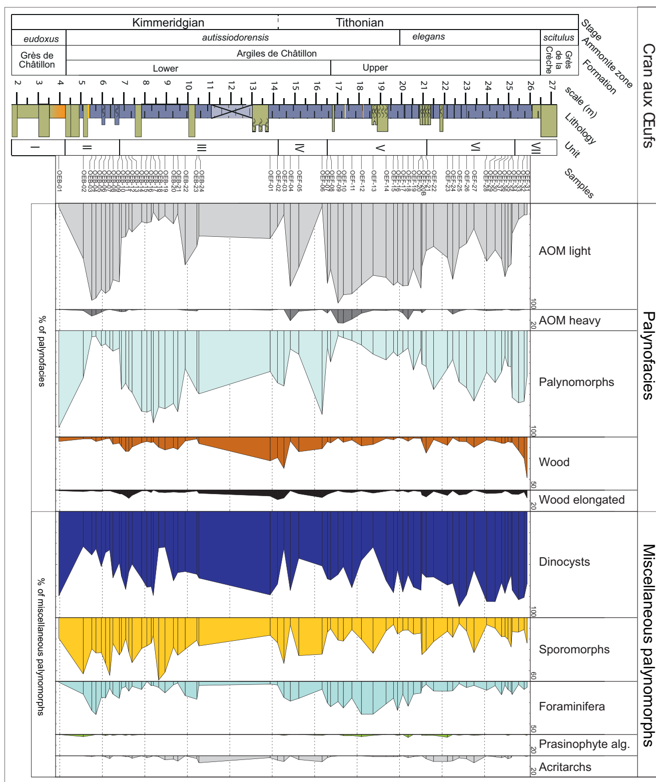
Fig. 10. (Colour online) Sawtooth percentage diagrams of the palynofacies counts and the miscellaneous palynomorph counts. On the left, the lithological column of the Cran aux Œufs section is displayed together with the individual samples and with the units that are used for the description of the results. AOM – amorphous organic matter.
