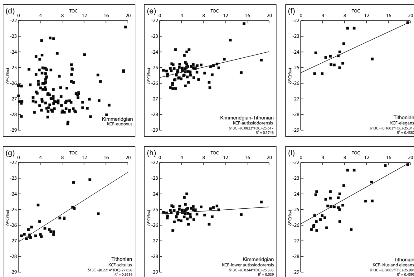
Fig. 7. \delta^{13}\text{C}_{\text{org}} against TOC plots for the ACF and KCF. (a) Lower and (b) upper ACF in the Cran aux Œufs section, and (c) the upper ACF in the Cap de la Crèche section. There is a clear positive correlation between \delta^{13}\text{C}_{\text{org}} and TOC in the upper ACF (b, c), which is absent in the lower ACF. In the KCF, \delta^{13}\text{C}_{\text{org}} against TOC plots for the (d) Eudoxus , (e) Autissiodorensis , (f) Elegans and (g) Scitulus ammonite zones display an increasing positive correlation with time. Plots for the age equivalent of the (h) lower and (i) upper ACF in the KCF based on \delta^{13}\text{C}_{\text{org}} correlations (Fig. 8) show, respectively, no correlation and a positive correlation.
