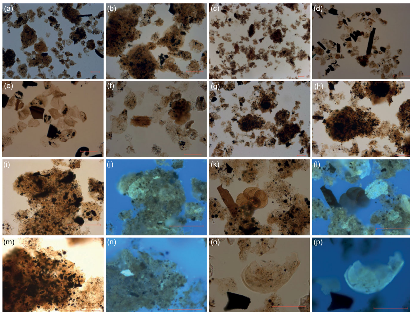
Fig. 13. (Colour online) Microphotographs of palynomorphs from the Argiles de Châtillon Formation. (a) Palynofacies from the lower OM-rich interval (sample OEB-03) showing dominant AOM; (b) same but with higher magnification. (c) Palynofacies from the upper OM-rich interval (sample OEF-10) showing dominant AOM. (d) Palynofacies from sample OEB-12, showing abundant wood particles. (e) Palynofacies from sample OEB-19, showing abundant sporomorphs. (f) Palynofacies from sample OEF-13 with a foraminiferal organic lining. (g) Palynofacies from sample OEF-03, showing heavy AOM. (h) Heavy AOM particle from sample OEF-03. (i) AOM particle from sample OEB-03; (j) the same AOM particle with incident UV light, showing an acritarch inside the particle. (k) Palynofacies from the lower OM-rich interval (sample OEB-03); (l) the same photograph but with incident UV light, showing a previously 'hidden' dinoflagellate cyst. (m) AOM particle from sample OEF-03; (n) the same particle with incident UV light. (o) An unidentifiable dinoflagellate cyst from sample OEF-13; (p) the same specimen with incident UV light. Scale bars = 50 µm.
