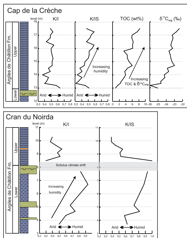
Fig. 14. (Colour online) Upper: Correlation of TOC and climate trends in clay mineral assemblages (kaolinite/illite and kaolinite/illite–smectite) of Tribovillard et al. (2019) for the Cap de la Crèche section. There is a clear large-scale positive correlation visible between TOC and humidity. Lower: Large-scale shift from humid climate below the sequence boundary to arid climate above the sequence boundary in Cran du Noirda. Note the higher values for the clay mineral ratios compared to those in Cap de la Crèche. The Scitulus climate shift is located within the sequence boundary, based on observations in the Cran aux Œufs record.
