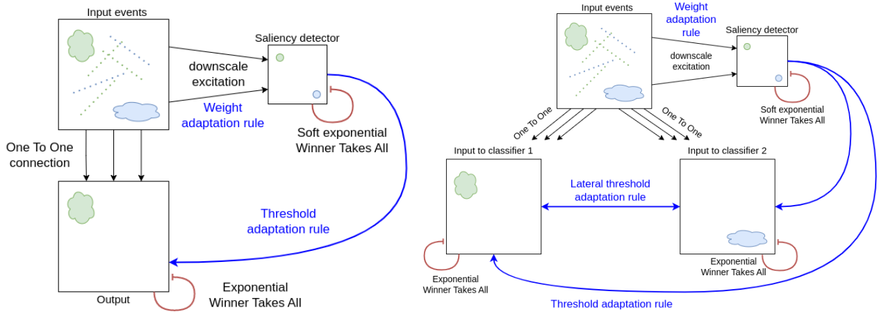
(a) Architecture of our initial neuromorphic model detecting saliency by event density and filtering out one OoI.
