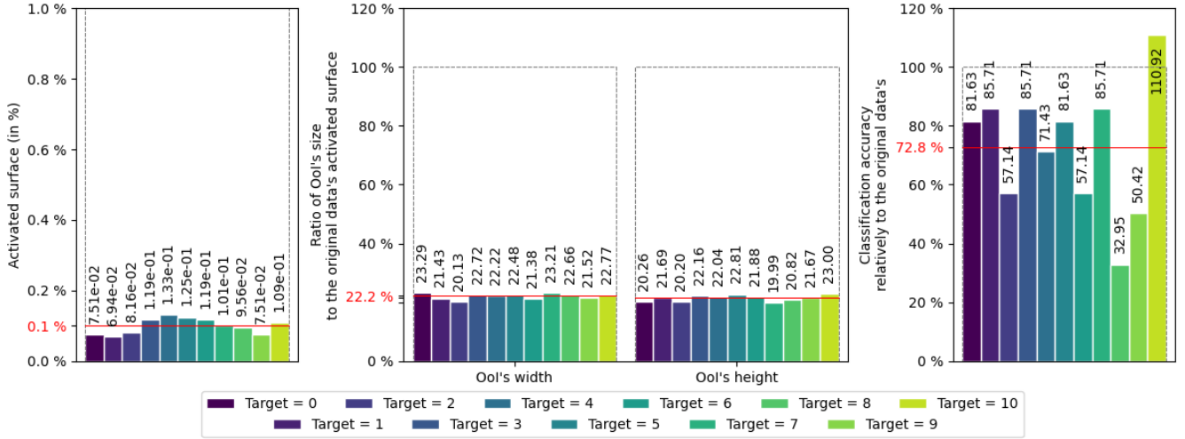
FIGURE 3 – Evolution of quantitative and qualitative properties of the DVS 128 Gesture dataset after attentional filtering, according to the dataset’s various targets i.e. various labelled gestures.
