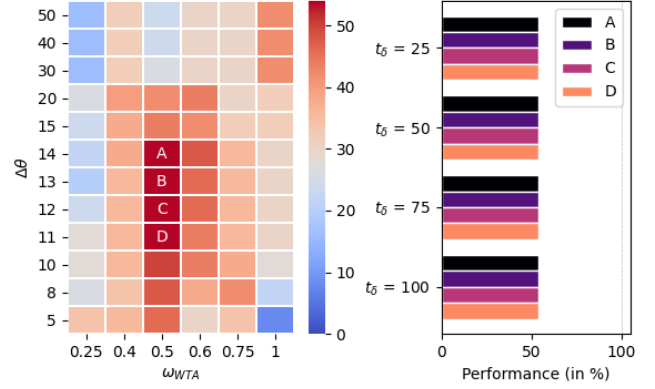
FIGURE 5 – Performance of simultaneous multi-OoIs detection according to the parameters \omega_{WTA} , \Delta\theta and t_\delta . The impact of t_\delta variation was observed for the parameterizations A ( \omega_{WTA} = 0.5 , \Delta\theta = 14 ), B ( \omega_{WTA} = 0.5 , \Delta\theta = 13 ), C ( \omega_{WTA} = 0.5 , \Delta\theta = 12 ) and D ( \omega_{WTA} = 0.5 , \Delta\theta = 11 ).
