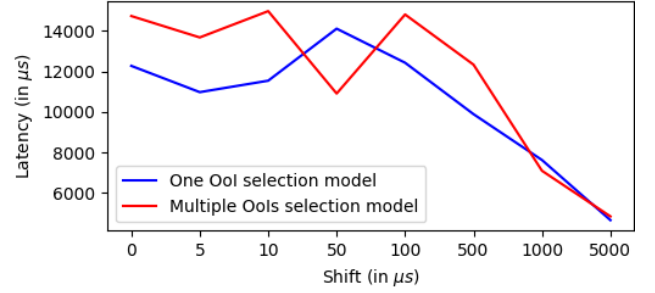
FIGURE 6 – Latency of the OoI selection in [5]'s (in blue) and our novel architecture according to the shift (in red). With the exception of the dip observed for a 50\mu s shift, the overall latency of OoI selection increases with the number of OoIs to be detected (from one in blue to two in red).
