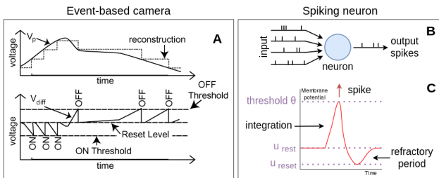
FIGURE 1 – (A) Principle of operation of an event-based camera, from [4]. (B) Behaviour of a spiking neuron, which receives spike trains as input and processes this information to produce a new sequence of activations. (C) Evolution of the neuron's membrane potential over time when activated by input spikes.
