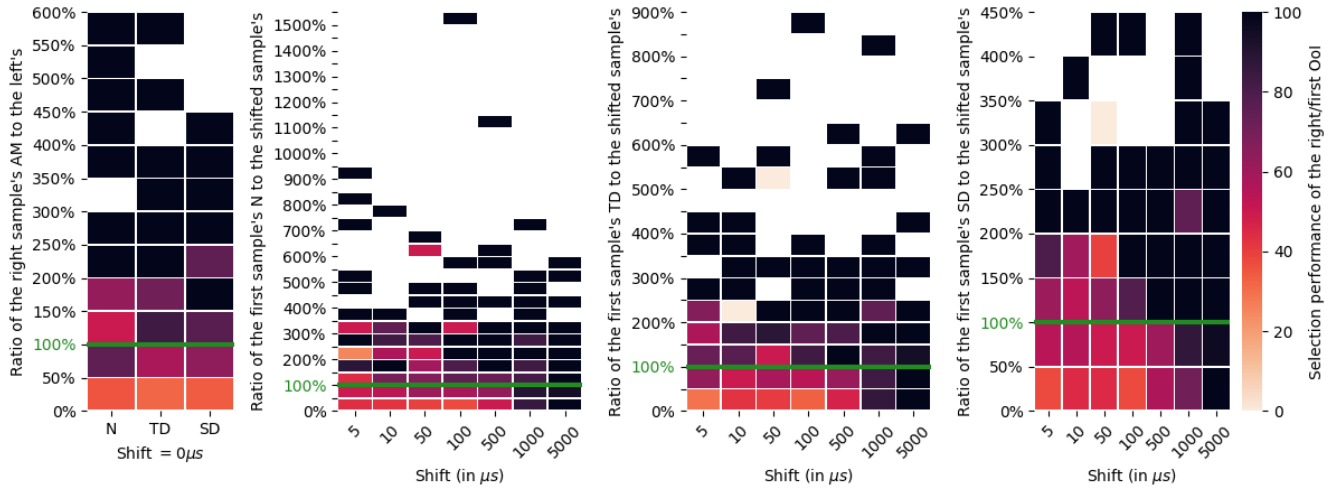
FIGURE 4 – Performance of the attentional filtering introduced in [5] according to the shift and diverse activity measures. N corresponds to the number of events, TD to the temporal density and SD to the spatial density.
