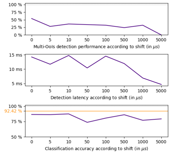
FIGURE 7 – Multi-OoIs detection performance (top), latency of the OoIs detection (middle) and classification accuracy of the selected OoIs (bottom) of the multi-OoIs selection model on a "control" dataset.
