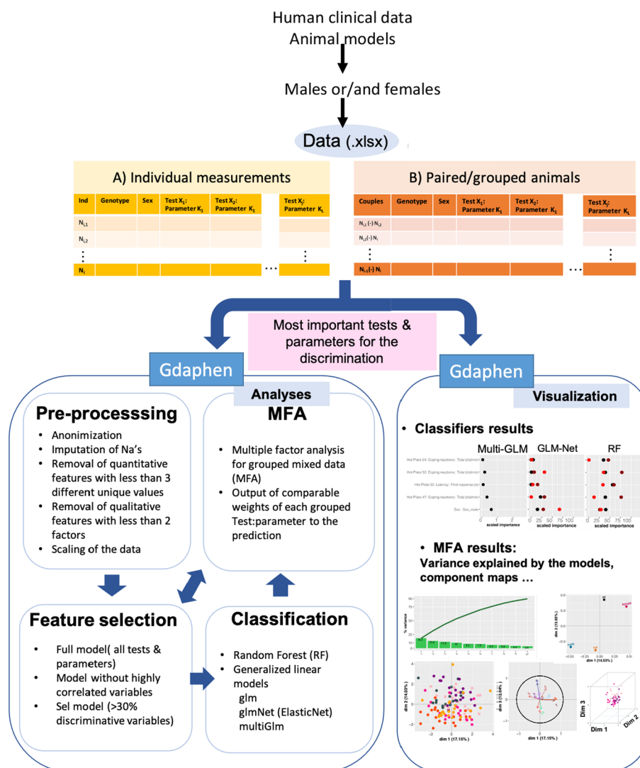
Fig. 1 Gdaphen workflow. Scheme highlighting the functionalities that Gdaphen can help to implement. From the data organized with individuals in rows and parameters measured in columns, Gdaphen comprises three modules. The first module deals with data pre-processing to shape the data in the input needed to perform the different analyses. Next, the module Analysis is where MFA, feature selection and classification strategies are performed. Last, the module visualization contains the functions that will generate the plots ready for the publications. As shown in the figure, a dotplot is implemented to show the classifiers results in the importance of each variable to the discrimination of your variable of interest. Then the MFA results are shown using different visualizations
