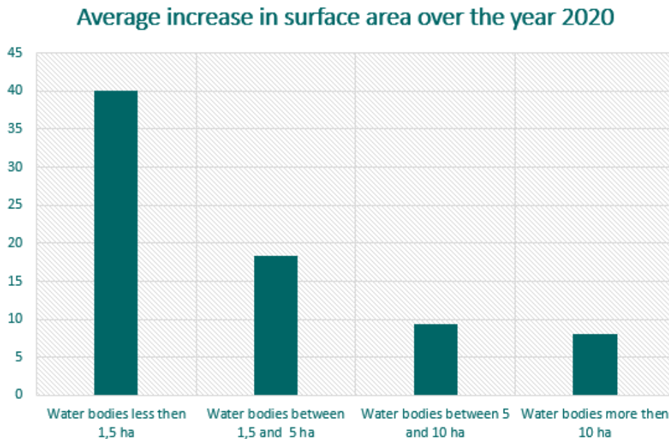
Fig. 10. Average increase in the surface of water bodies between the 5 meter and 10 meter detection, by categories of areas in reference database.
