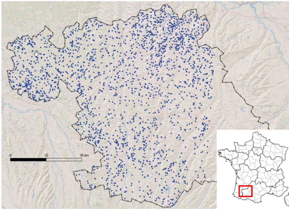
Fig. 9. Local reference database, build from photo-interpretation of Very High Resolution aerial photography (20 cm), corrected and completed by field campaigns, provided by local users of the Gers district, France.
