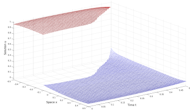
Fig. 10: Graph of the approximate solution \widetilde{u}_d(t, x, 0.6) for d = 5 without imposing (18)
