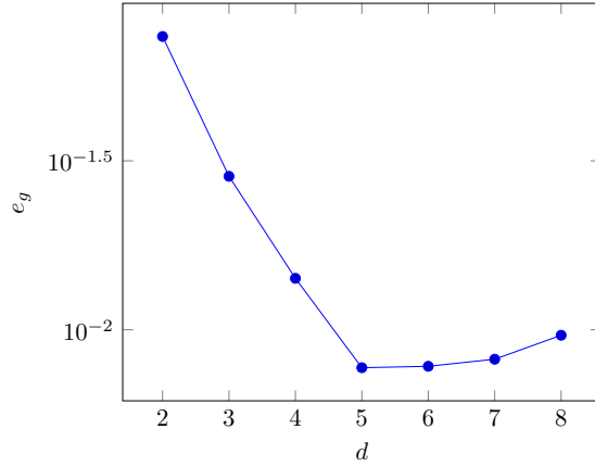
Fig. 9: Evolution of the error e_g with relaxation degree d
