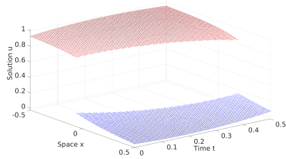
(a) d = 2
