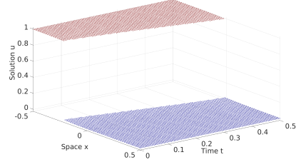
(b) d = 5
