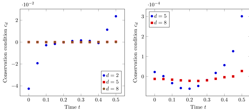
Fig. 10: Conservation condition c_d(t, 0.2) versus time t for d = 2, 5, 8 (left) and for d = 5, 8 (right)
