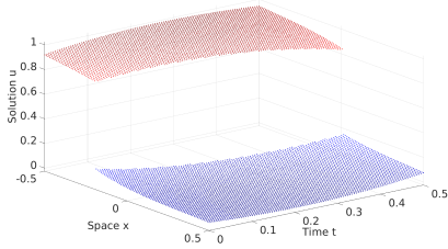
(a) d = 2
