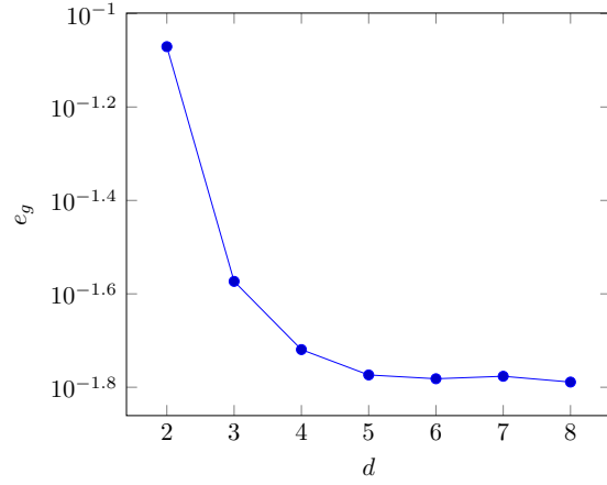
Fig. 3: Evolution of the error e_g with relaxation degree d
