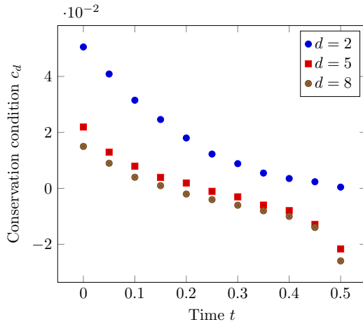
Fig. 6: Conservation condition c_d(t, 0.2) versus time t for d = 2, 5, 8
