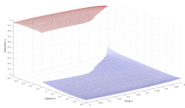
Fig. 11: Graph of the approximate solution \widetilde{u}_d(t, x, 0.6) for d = 5 without imposing (18)
