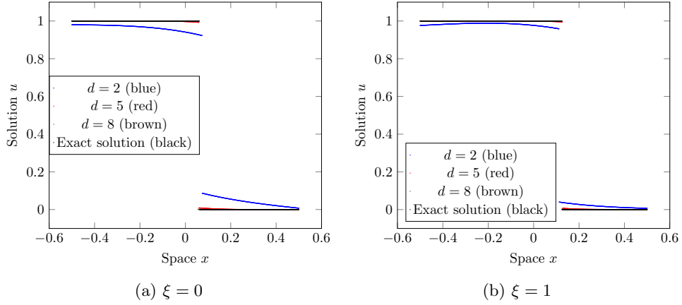
Fig. 8: Graphs of the approximate solution \widetilde{u}_d(\frac{1}{4}, x, \xi) for d = 2, 5, 8 , superposed with the exact solution
