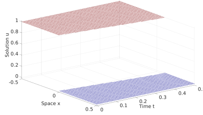
(c) d = 8
