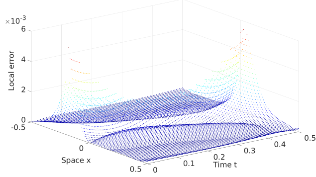
Fig. 5: Graph of the error \varepsilon(t, x) = |\widetilde{u}_5(t, x, 0.2) - u(t, x, 0.2)|
