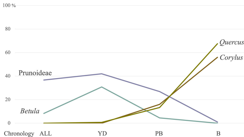
Figure 10: Relative frequencies of the dominant taxa (whose variations are statistically significant) throughout the studied sequence correlated with the associated chronozone.
