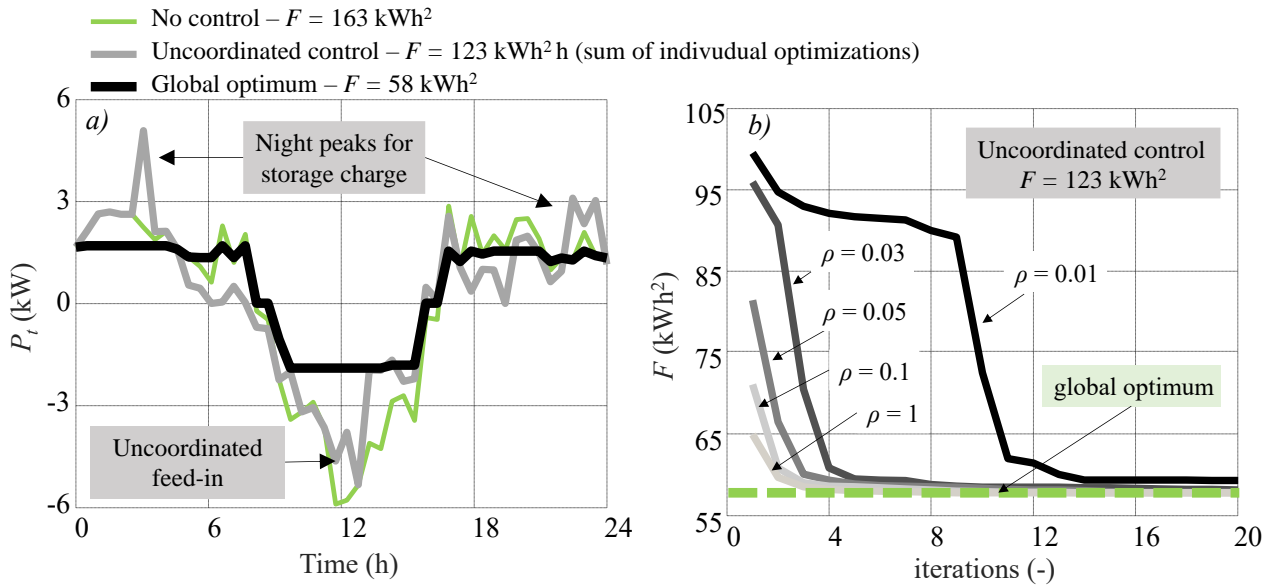
Figure 4: a) Aggregated grid power – global optimum and solution with no storage or uncoordinated storage control. b) Global objective decrease along the iterations for different convergence rate values.
