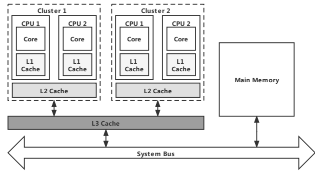
Figure 1: An example multi-core architecture with a three-layered cache hierarchy.
