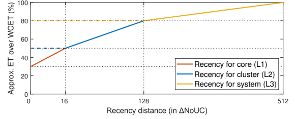
Figure 4: An illustrative cache recency profile.
