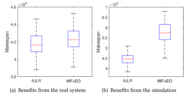
Figure 6: The makespan (in microseconds) of AJLR and WF+EO on (a) the real system and (b) the simulator.
