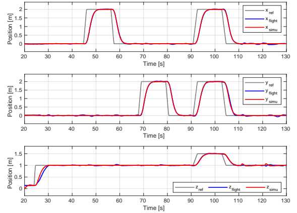
Figure 9: Positions response in case of no Magnus rotation
