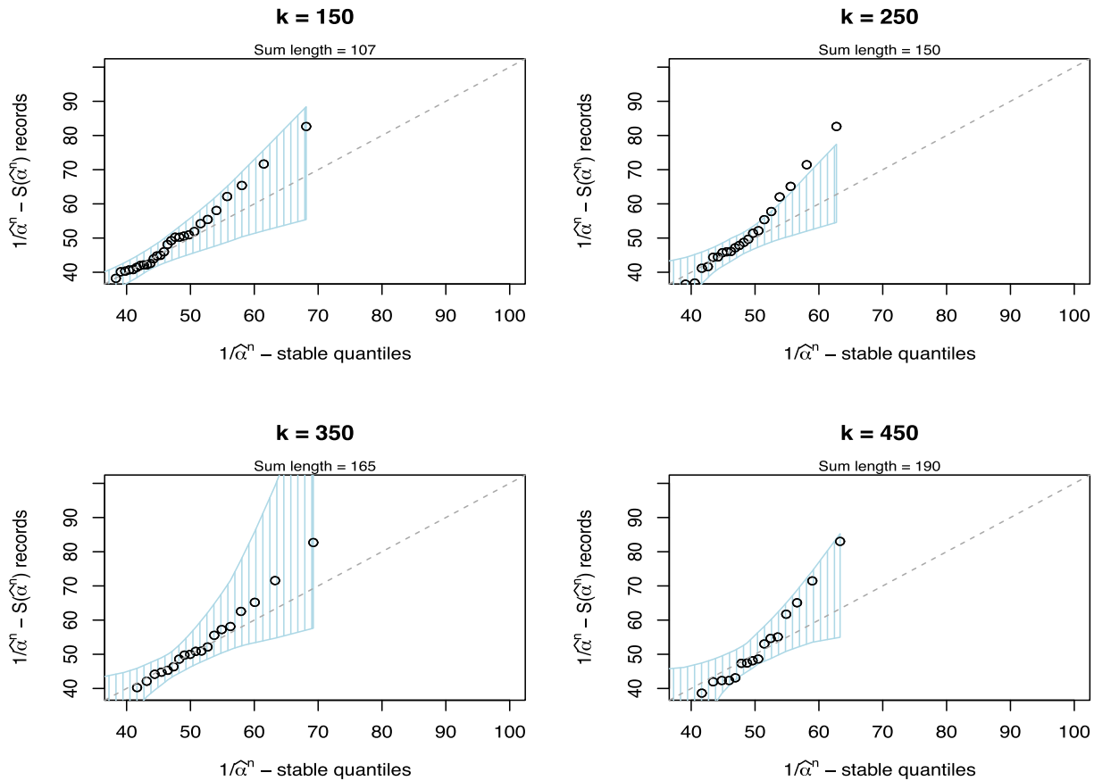
FIGURE 6 qqplots for different k values of the 1/\hat{\alpha}^n(k) -stable quantiles against the 1/\hat{\alpha}^n(k) - (S_{t,b}(\hat{\alpha}^n(k)))_{t=1, \dots, \lfloor n/b \rfloor} records with 95% confidence intervals for the northwest.
