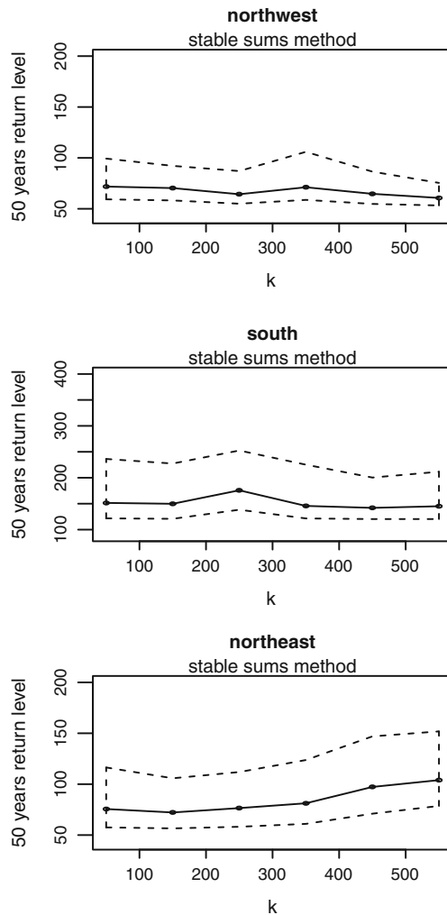
FIGURE 5 Estimates of the 50 years return level of fall supremum norm observations with confidence intervals. We write estimates as a function of k with the parametrization detailed in Section 5.1.
