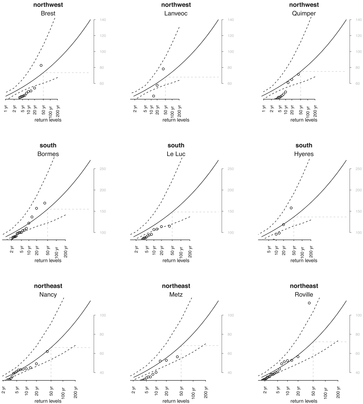
FIGURE 9 Return level plots with confidence intervals based on 1000 bootstrap replicates. The grey dotted line gives the estimated 50 years return level. Other return levels can be obtained alike. The black line is the \log(x) \mapsto x plot. The points are the logarithm of estimated 1/\hat{\alpha}^n -stable quantile at (1 - \frac{k}{n \hat{m}^{(j)}})^{b_n} versus the k th largest order statistics; see Equation (17). The largest order statistics should lie on the solid line.
