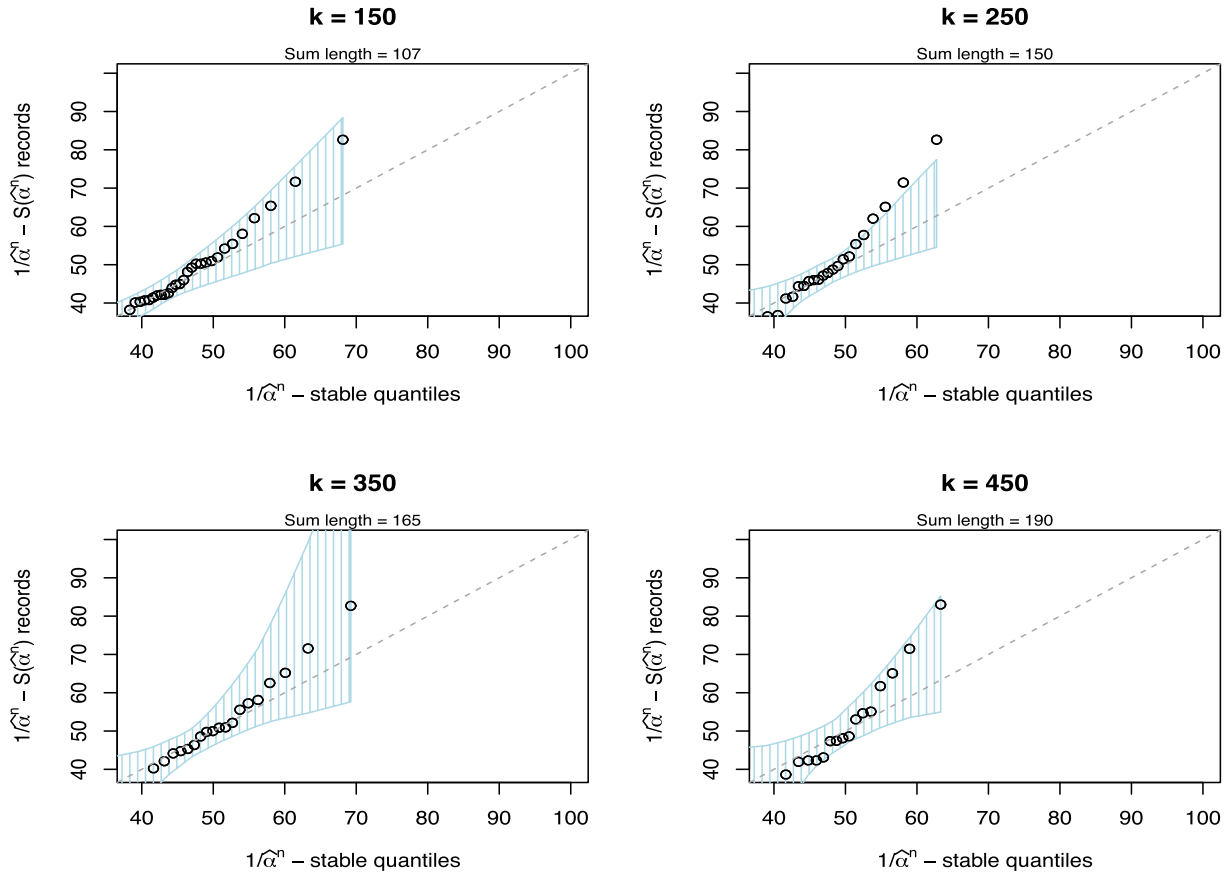
FIGURE 6 qqplots for different k values of the 1/\hat{\alpha}^n(k) -stable quantiles against the 1/\hat{\alpha}^n(k)-(S_{t,b}(\hat{\alpha}^n(k)))_{t=1, \dots, \lfloor n/b \rfloor} records with 95% confidence intervals for the northwest.
