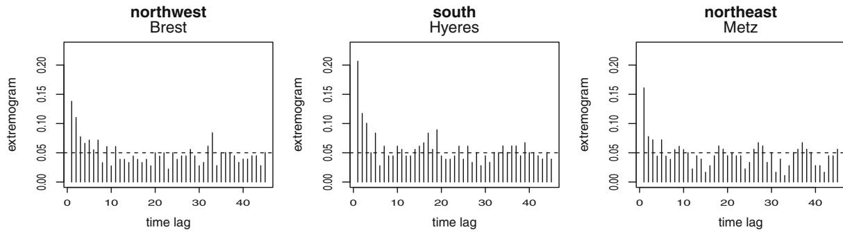
FIGURE 2 Empirical temporal extremogram of the 95th order statistic of fall daily rainfall in France from 1976 to 2015. The first, middle, and last correspond to three climatological regions as in Figure 1. As a baseline, the extremogram takes the value indicated by the dotted line on independent time lags.
