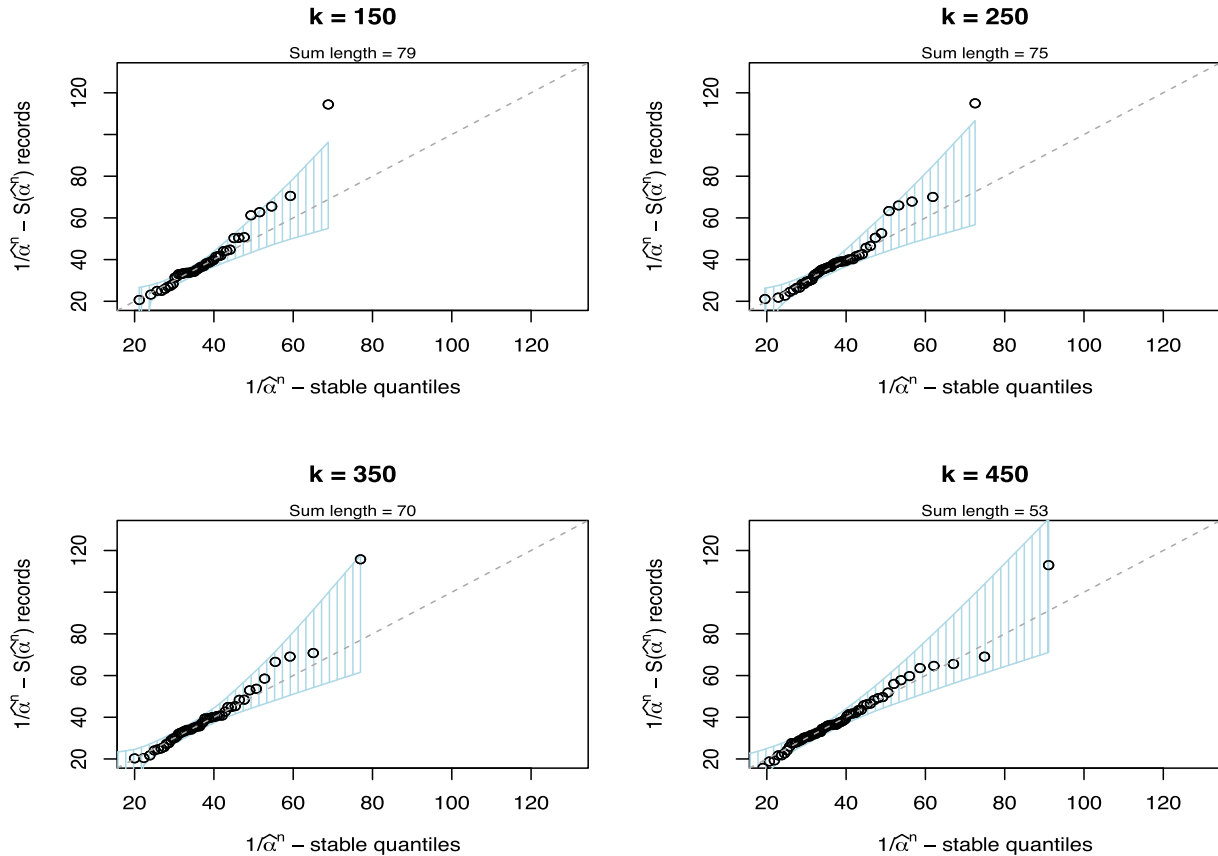
FIGURE 8 qqplots for different k values as in Figure 6 but for the northeast region.
