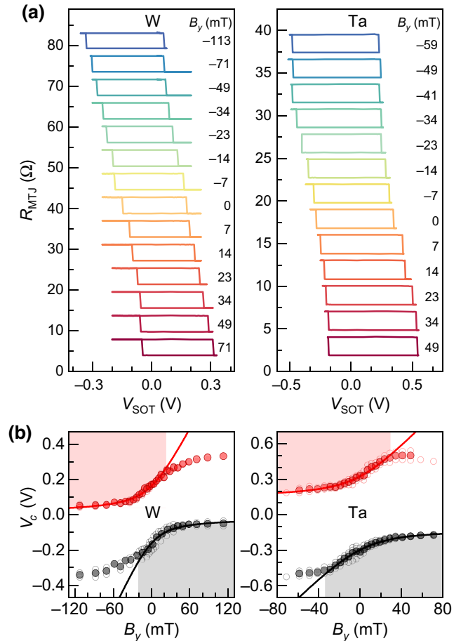
FIG. 3. (a) Switching loops of W- and Ta-based MTJ for different B_y at constant |B_x| = 40 mT. The MTJ resistance is measured as a function of V_{\text{SOT}} after applying a current pulse with t_p = 1 ms. The measurements are offset along the y axis for clarity. (b) Critical switching voltage as a function of B_y . The full symbols show the average of the individual V_c (open symbols) measured at positive and negative B_x . The lines are fits to the data (see text) in the range marked by the shaded areas.
