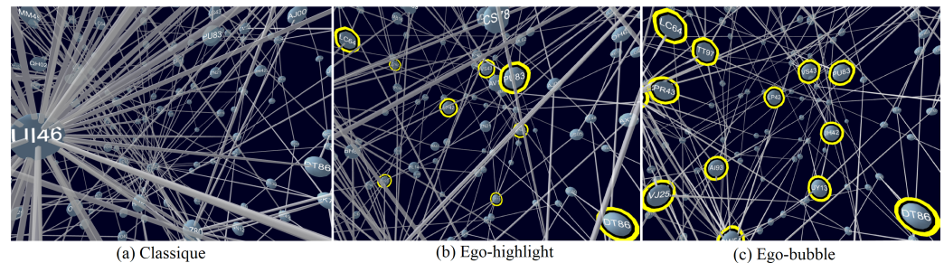
Figure 4. Immersive exploration of the node's neighbors. (a) Classic: the user inspects the UI46 node up close. (b) Ego-highlight: the user takes the position of the UI46 node, with direct neighbors highlighted in yellow. (c) Ego-bubble: direct neighbors are positioned equidistant from the user. (Images taken from Sorger et al. [21]).
