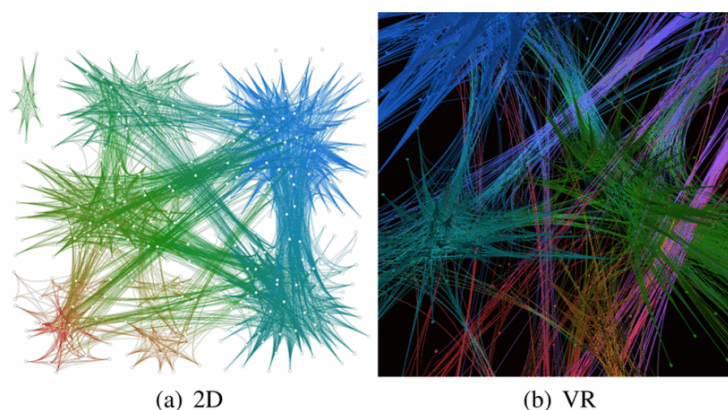
Figure 3. In this 2D visualization, the entire graph may be visible, but it is difficult to discern the connectivity of certain nodes. In the immersive environment, only a small section of the graph is visible at any given time, but the structure is more tangible. (Image is from Kwon et al. [17], © 2015, IEEE).
