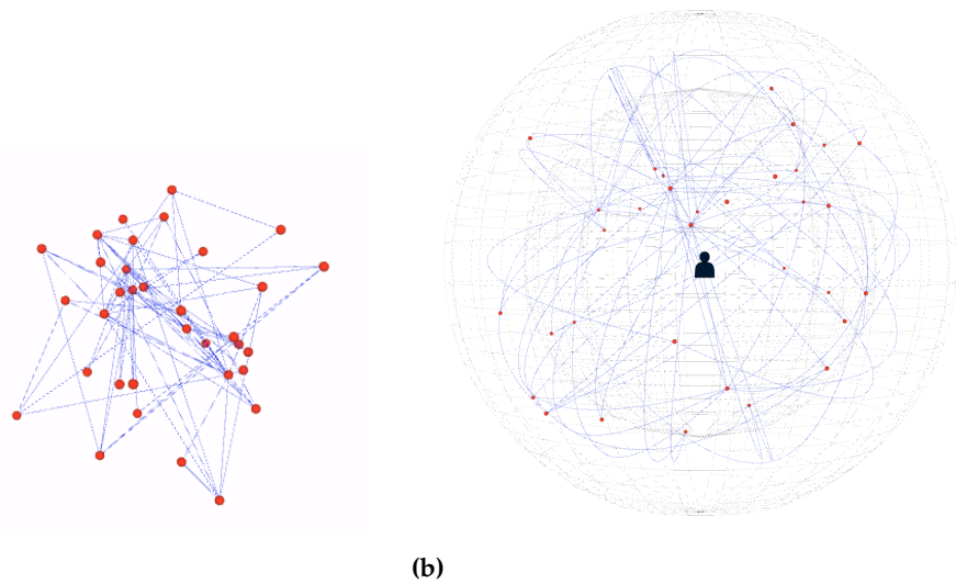
Figure 6. Visualization of the karate club graph (34 nodes and 78 edges) [24]. (a) visualization using Fruchterman and Reingold’s algorithm; (b) our egocentric metaphor where the graph is positioned between two concentric spheres.
