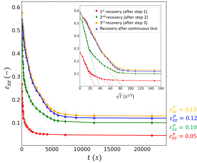
Figure 7: Main graph: evolution of the recovery strain \varepsilon_{zz}^{res} with time t for the various cycling steps used for the interrupted or the continuous cycling procedures. The inset gives a zoom of the early stages of the recovery processes as a function of \sqrt{t} .
