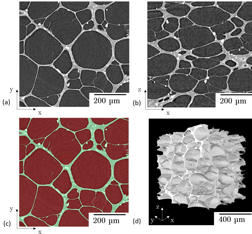
Figure 2: 2D slices orthogonal (a) or parallel (b) to the compression axis z of an underformed foam sample. Slice (a) (in c) and 3D view of the ROI (d) after proper segmentation using the weka segmentation plugin.
