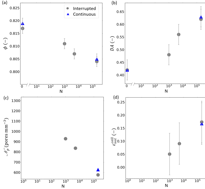
Figure 10: Structural evolution during the interrupted (●) and the continuous (▲) cycling procedures as function of the number of compression cycles N : (a) porosity \phi , (b) average degree of anisotropy of cell DA , (c) apparent volumetric number of pores \mathcal{N}_p , (d) cell volume strain \epsilon_{vol}^{cell} .
