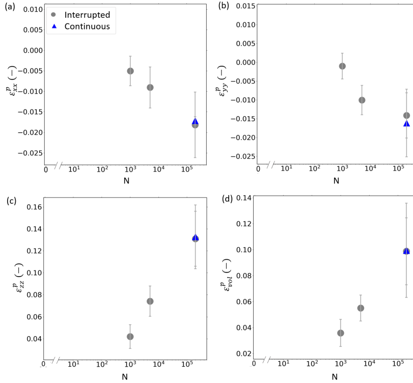
Figure 8: Evolution of the strain components perpendicular ( \varepsilon_{xx}^p (a), \varepsilon_{yy}^p (b)) and parallel ( \varepsilon_{zz}^p , (c)) to the compression direction z and of the volume strain \varepsilon_{vol}^p (d) as functions of the number of cycles N , recorded during the interrupted (●) and the continuous (▲) cycling procedures.
