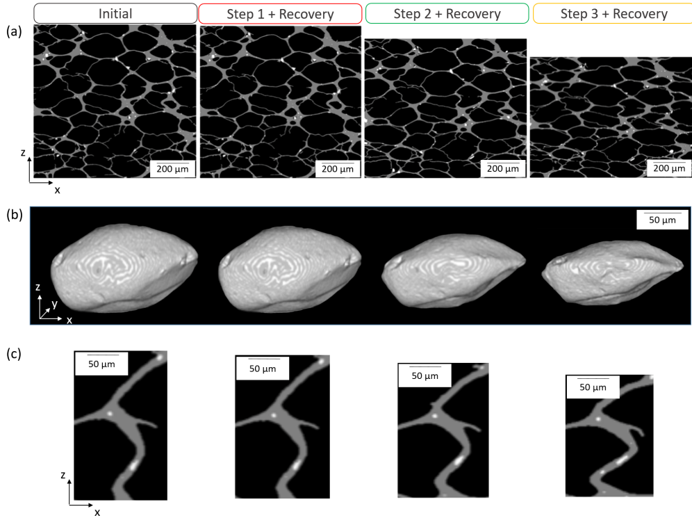
Figure 9: Structural characterization during ex situ interrupted fatigue procedure obtained by X-ray microtomography, (a) at the foam scale, (b) at the cell scale, (c) at the cell-wall scale.
