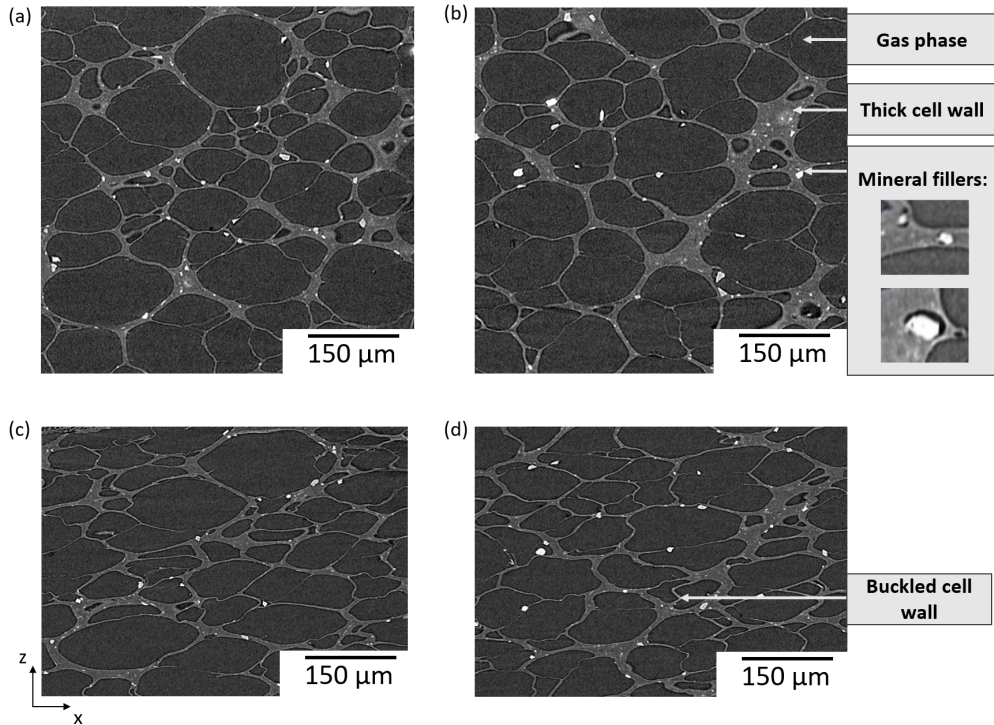
Figure 4: Slices of the initial microstructures of samples used for the (a) interrupted and the (b) continuous cycling procedures. Same microstructures (after image registration) corresponding to the (c) interrupted and to the (d) continuous procedures at the end of cycling, i.e. , at N = 200000 .
