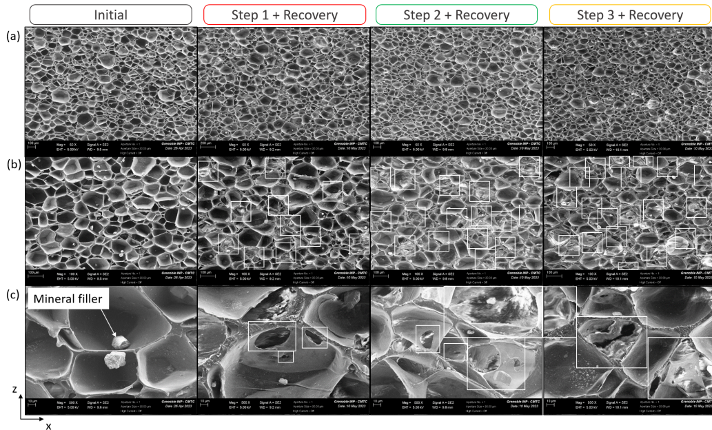
Figure 12: Structural characterization during ex situ interrupted fatigue procedure obtained by SEM, (a) at the sample scale, (b) at the cell scale, (c) at the wall scale. White frames point out the teared cell walls.
