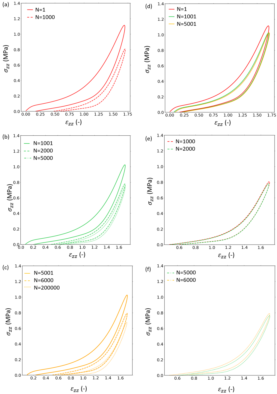
Figure 5: Stress-strain curves of EVA foam during (a) step 1, (b) step 2 and (c) step 3 of the interrupted procedure. Comparison of (d) the 1 st cycles of step 1, 2 and 3, (e) the last cycle of step 1 with the 1000 th cycle of step 2, (f) the last cycle of step 2 with the 1000 th cycle of step 3.
