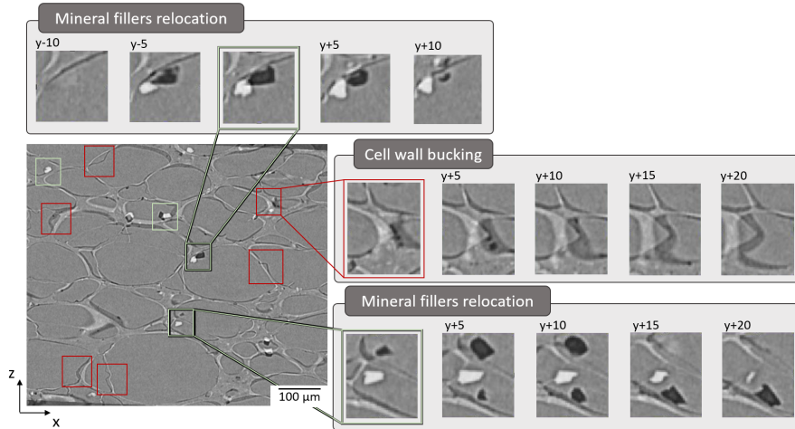
Figure 11: Slice showing the difference between the initial 3D image and the final registered 3D one. When both images perfectly overlap on one voxel, the resulting value is 0 and appears gray. Values that are highly positives ( i.e. , the lighter zones) are associated to the initial image, whereas values that are highly negatives ( i.e. , the darker zones) correspond to the final image. The reported slices highlight the relocation of the mineral charges initially put onto the cell wall and the cell wall bending induced during cycling.
