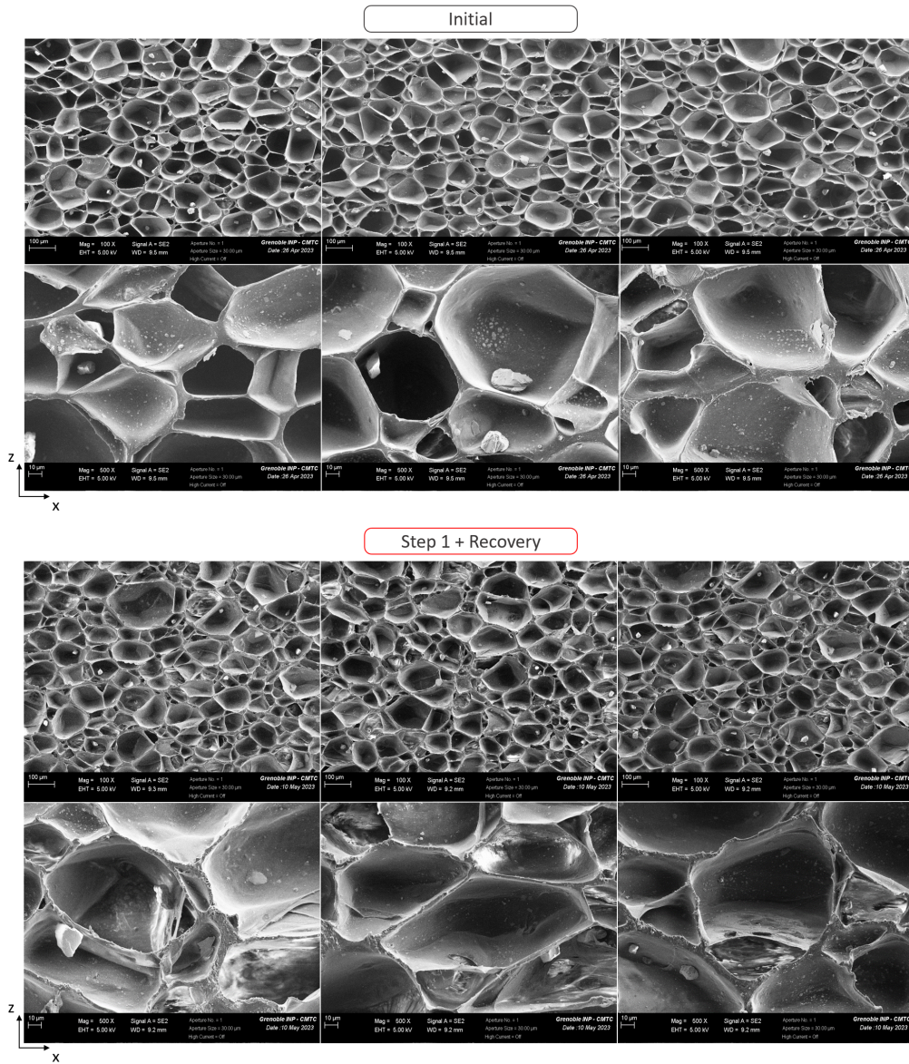
Figure 13: Additional structural characterization during ex situ interrupted fatigue procedure obtained by SEM at the cell scale and at the wall scale for the initial microstructure and for the microstructure after the first fatigue step and recovery.
