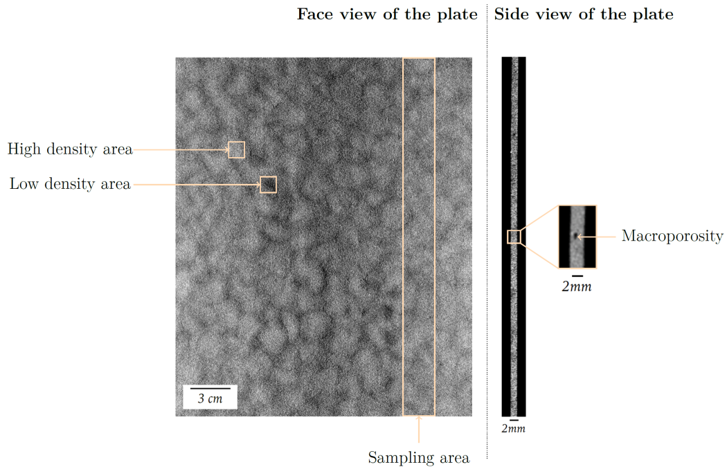
Figure 3: Orthogonal slices showing the in-plane (left) and the out-of-plane (right) macroscale heterogeneities in the core of the tested slab produced by compression molding.
