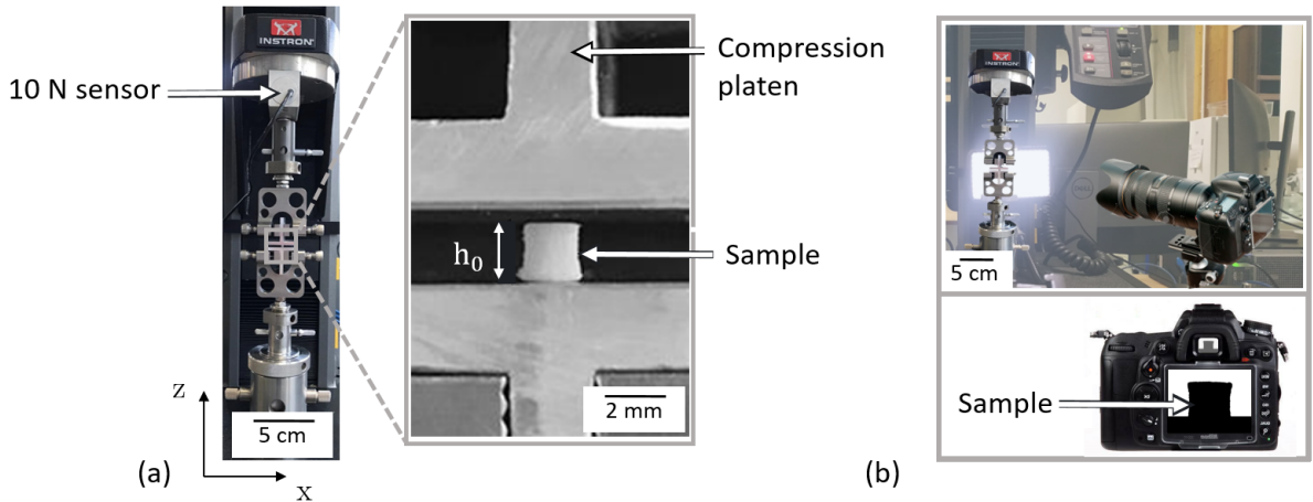
Figure 1: (a) Compression device with a zoom on a sample mounted between the compression platens. (b) View of the the set-up used to estimate the recovery strain after cycling (led screen placed behind the sample + camera).
