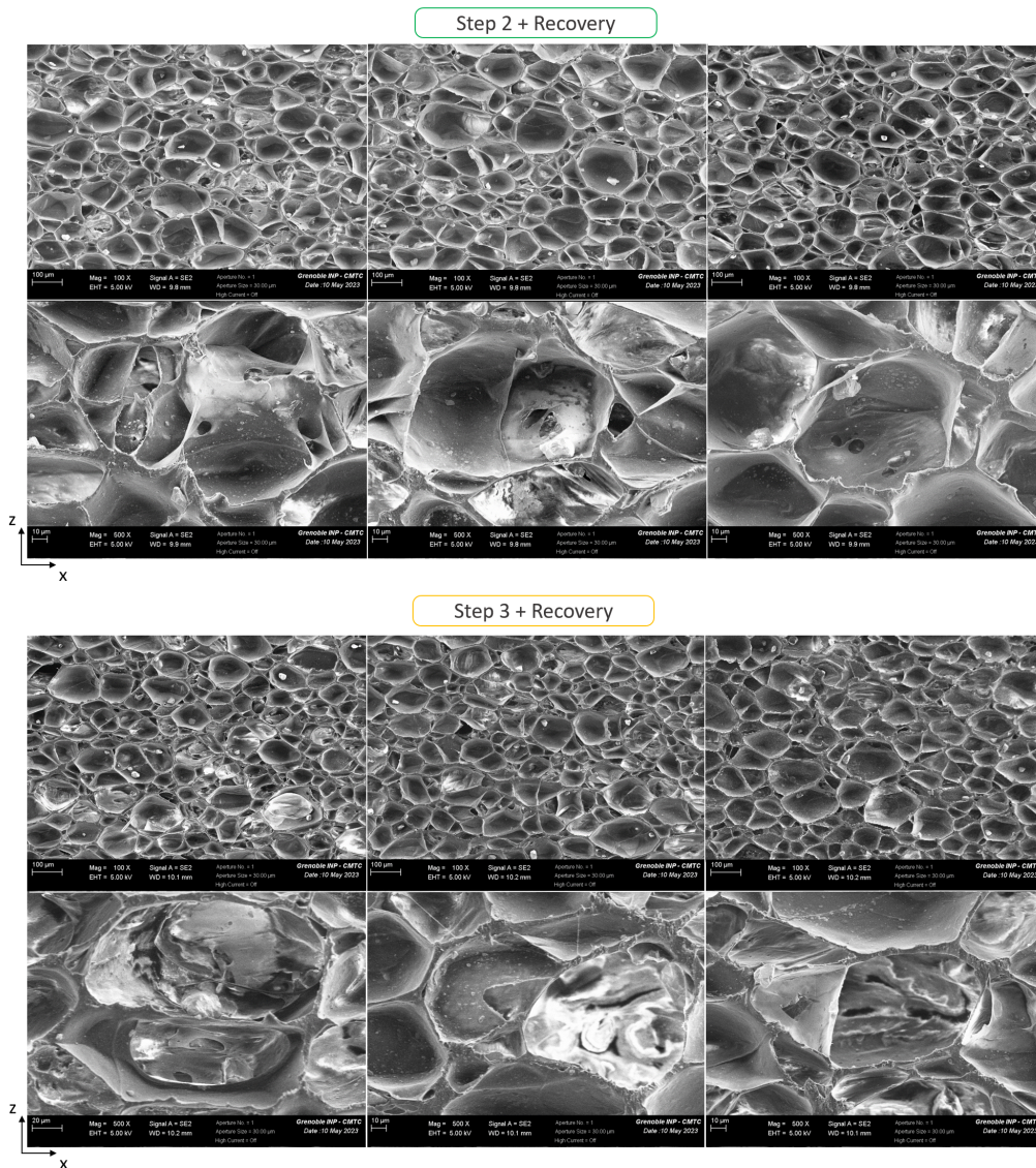
Figure 14: Additional structural characterization during ex situ interrupted fatigue procedure obtained by SEM at the cell scale and at the wall scale for the microstructure after the second and the third fatigue step and recovery.
