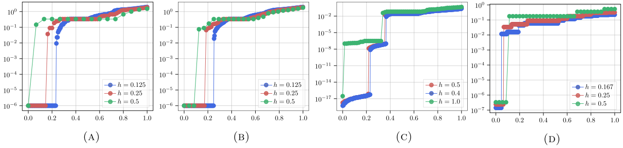
FIGURE A.2. Eigenvalues of \mathcal{S}_{\mathcal{F}\mathcal{F}} on different meshes for polynomial orders (0,0). (a) Right triangles. (b) Unstructured triangles. (c) Unstructured tetrahedra. (d) Cartesian hexahedra.
