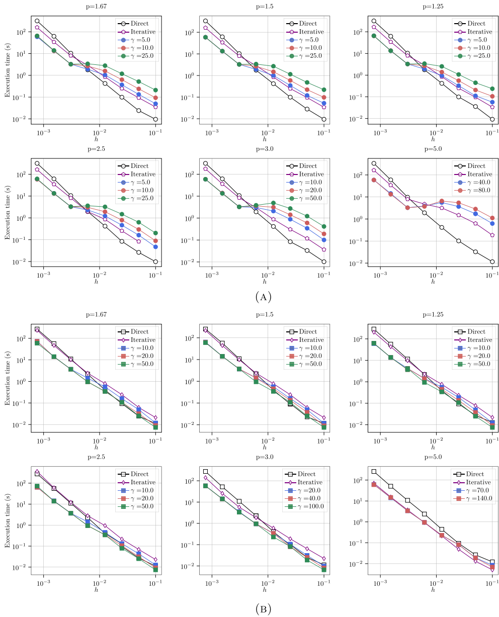
FIGURE 10. Nonlinear ( p -structure) wave problem with p \in \{1.25, 1.5, 1.67, 2.5, 3, 5\} - Comparison of execution times for a single time step of the splitting procedure and of the semi-implicit scheme (with either a direct or an iterative solver), polynomial orders (1, 1) and (2, 1). (a) (1, 1). (b) (2, 1).
