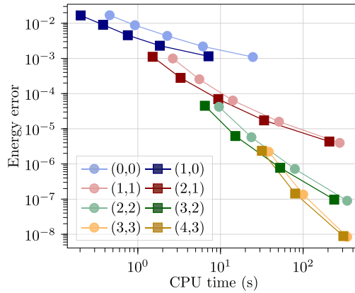
FIGURE 5. Linear wave problem - Energy error with optimal \gamma as a function of the execution time, with (k, \gamma) \in \{(0, 9), (1, 22.5), (2, 42), (3, 67.5)\} in the equal-order setting and (k, \gamma) \in \{(0, 1), (1, 45), (2, 84), (3, 135)\} in the mixed-order setting.
