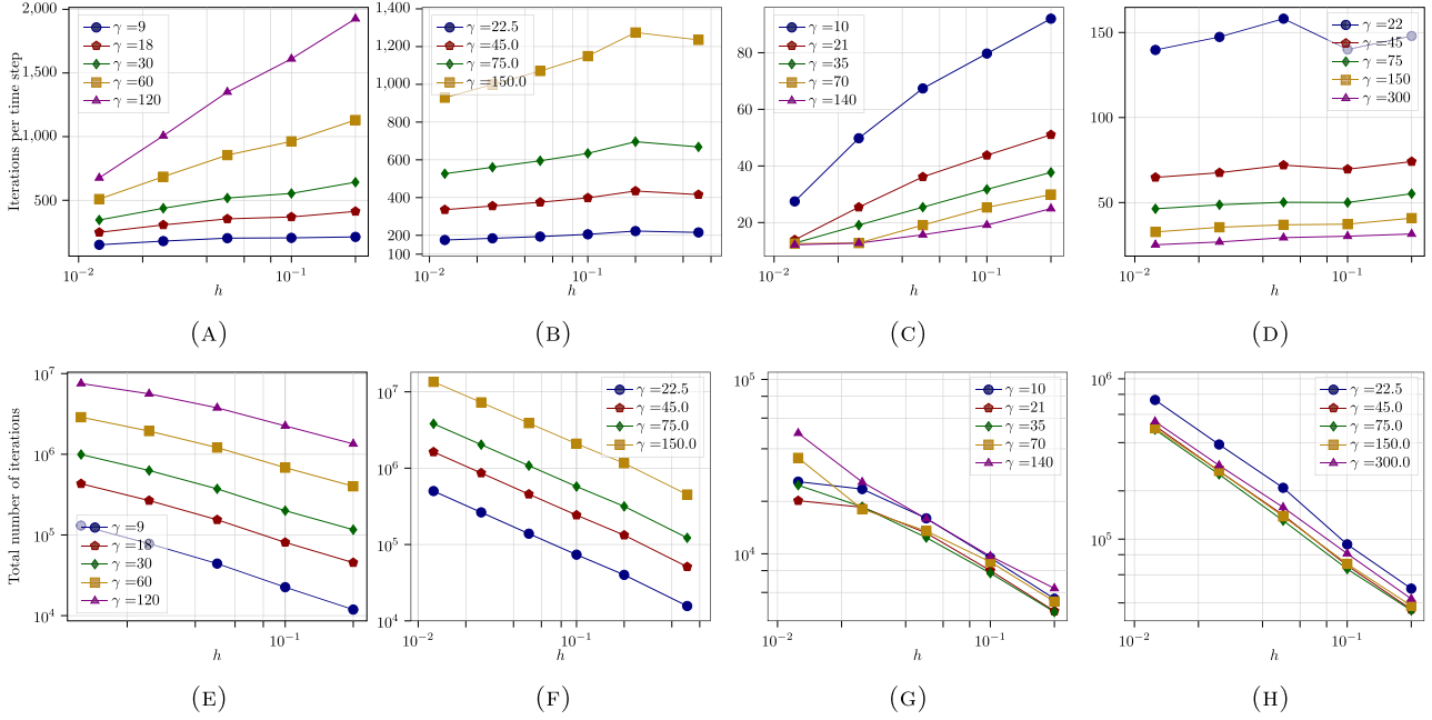
FIGURE 4. Linear wave problem - Mean number of splitting iterations per time step (top) and total number of splitting iterations in log scale (bottom), as a function of the mesh size, k \in \{0, 1\} , equal- and mixed-order settings. (a) (0, 0). (b) (1, 1). (c) (1, 0). (d) (2, 1). (e) (0, 0). (f) (1, 1). (g) (1, 0). (h) (1, 1).
