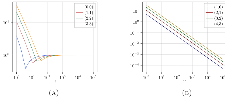
FIGURE A.3. Spectral radius of the iteration matrix as a function of \gamma , equal-order setting (left) and mixed-order setting (right) on an unstructured triangular mesh with h = 0.1 . (a) Equal-order. (b) Mixed-order.
