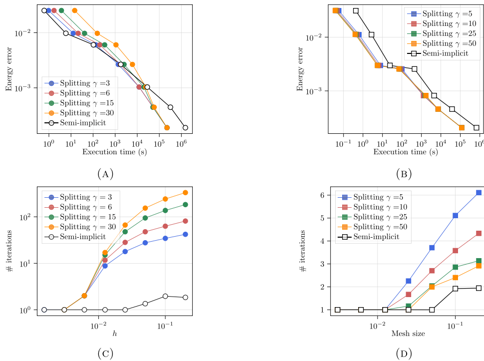
FIGURE 7. Nonlinear (p-structure) wave problem with p = 3 - Energy error as a function of execution time (top) and mean number of iterations per time step as a function of mesh size (bottom), \gamma \in \{\gamma^{\min}, 2\gamma^{\min}, 5\gamma^{\min}, 10\gamma^{\min}\} , polynomial orders (0,0) and (1,0). (a) (0,0). (b) (1,0). (c) (0,0). (d) (1,0).
