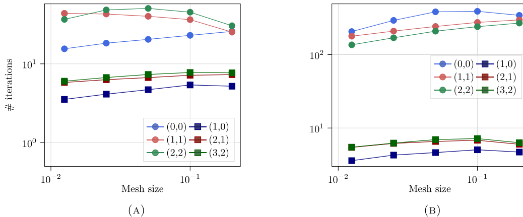
FIGURE 13. Vibrating membrane with \alpha \in \{0.8, 0.99\} - Mean number of iterations per time step for polynomial orders k \in \{0, 1, 2\} , mixed- and equal-order settings, with splitting (only the best value of \gamma is displayed). (a) \alpha = 0.8 . (b) \alpha = 0.99 .
