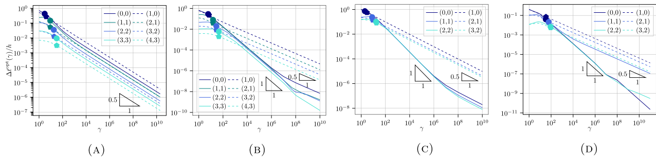
FIGURE A.4. Ratio \frac{\Delta t^{\text{opt}}(\gamma)}{h} as a function of \gamma on 2D and 3D unstructured meshes. (a) Quadrangles. (b) Triangles. (c) Hexahedra. (d) Tetrahedra.
