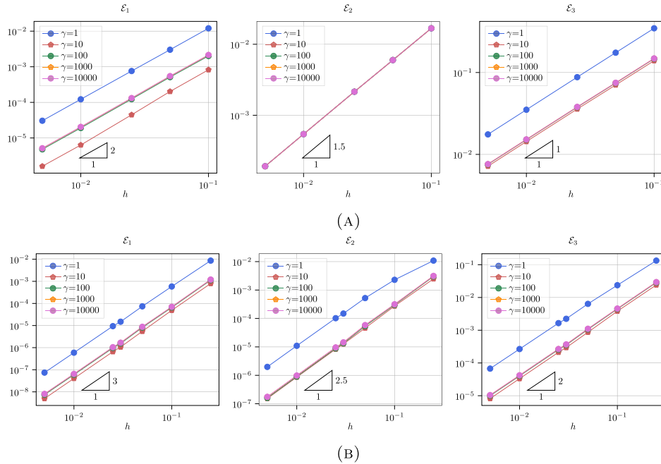
FIGURE A.1. Errors \mathcal{E}_1, \mathcal{E}_2, \mathcal{E}_3 on the scalar Laplacian as a function of the mesh size for \gamma \in \{1, 10, 100, 1000, 10000\} , equal-order setting with k \in \{0, 1\} . (a) (0, 0) . (b) (1, 1) .
