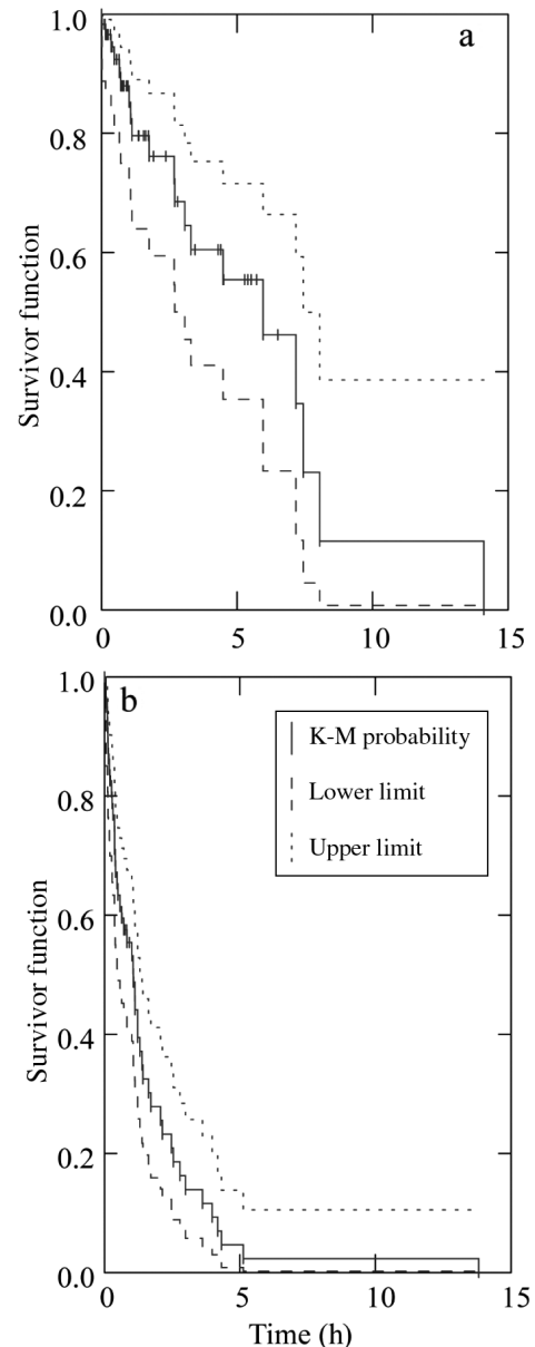
Fig. 5. Eubalaena glacialis . Kaplan-Meier (K-M) survival plot for the maximum inter-call interval, including completely censored tag records (i.e. tag records with no whale calls): (a) survival plot for calls from the tagged whales and (b) survival plot for calls from any right whale recorded on the tag
