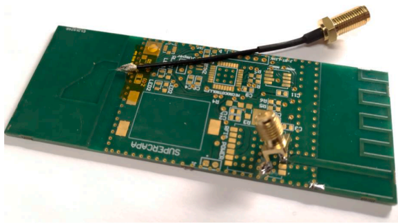
Fig. 9. SMA connector and coaxial cable soldered respectively to the feed point of IFA and slot antenna.
