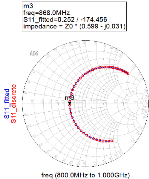
Fig. 8. Simulated input impedance of the IFA.
