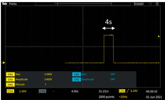
Fig. 15. Accumulator (supercapacitor) discharge time measurement.
