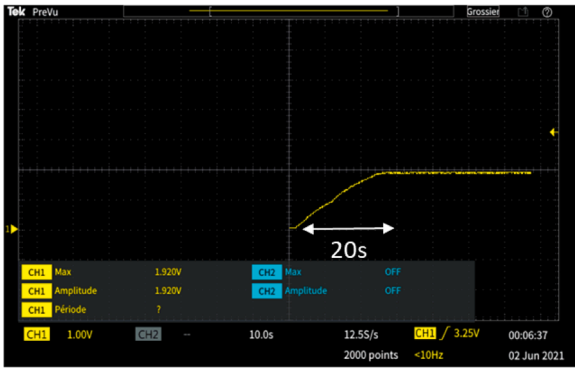
Fig. 14. Accumulator (supercapacitor) charging time measurement.
