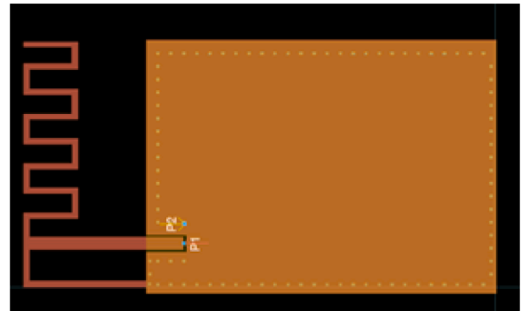
Fig. 3. Designed IFA antenna (75 × 40 mm 2 ).
