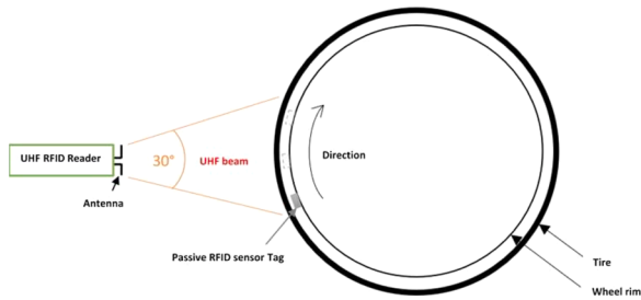
Fig. 1. Tag implantation synoptic on the bicycle wheel.
