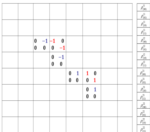
Figure 6 Color online. Matrix (\mathcal{L}_{1+} + \mathcal{L}_{2+})/(-i) in the case of a two-state system with two artificial decay modes and n_{max} = 1 . \mathcal{L}_{1+} in blue and \mathcal{L}_{2+} in red.
