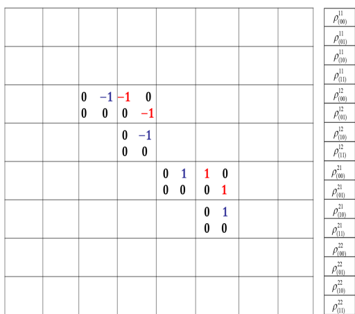
Figure 6 Color online. Matrix (\mathcal{L}_{1+} + \mathcal{L}_{2+})/(-i) in the case of a two-state system with two artificial decay modes and n_{max} = 1 . \mathcal{L}_{1+} in blue and \mathcal{L}_{2+} in red.
