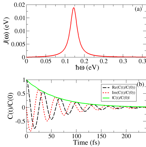
Figure 9 (a) Spectral density of the model presented in figure 8 to illustrate the population-to-coherence transfer. The spectral density maximum is close to the mean BD energy gap; (b) corresponding normalized correlation function C(t)/C(0) (Eq.(4)) at T = 298\text{K} with real part (dashed line), imaginary part (dots) and modulus (solid line).
