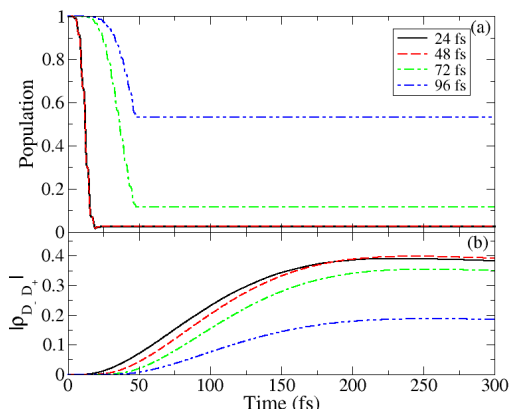
Figure 11 Excitation of the bright state B by a \pi pulse of different durations. (a) Population in the ground state, (b) Modulus of the coherence (\rho_S)_{D_+D_-} generated in the dark doublet .
