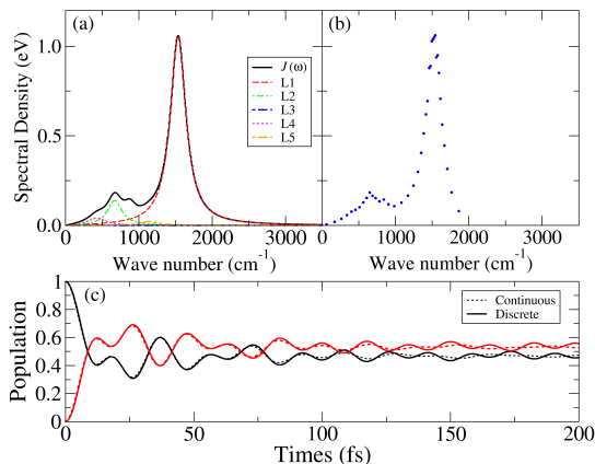
Figure 16 Excitation energy transfer dynamics with a continuous or discretized spectral density by the TT implementation. (a) : continuous spectral density fitted by five two-pole Lorentzian functions (Eq.(9)), see Refs.[67, 93], (b) : discretization in N_{disc} = 40 modes by the Makri procedure (see Ref.[137]) leading to K = 2N_{disc} decay modes, (c) : population in the XT (black) and CT (red) states when the initial state is XT. Dashed lines: TT implementation with the continuous spectral density leading to K = 10 decay modes without Matsubara terms at 298 K; solid lines : TT implementation with K = 80 discrete modes .
