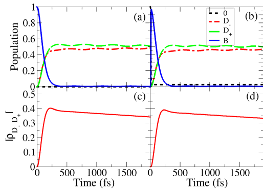
Figure 10 Upper panels: populations in the eigenstates B , D_- and D_+ , (a) ideal preparation in the bright state B , (b) excitation of the B state from the ground state by a \pi pulse of 24 fs. lower panels: modulus of the coherence (\rho_S)_{D_+D_-} , (c) ideal preparation in the bright state, (d) excitation by a \pi pulse.
