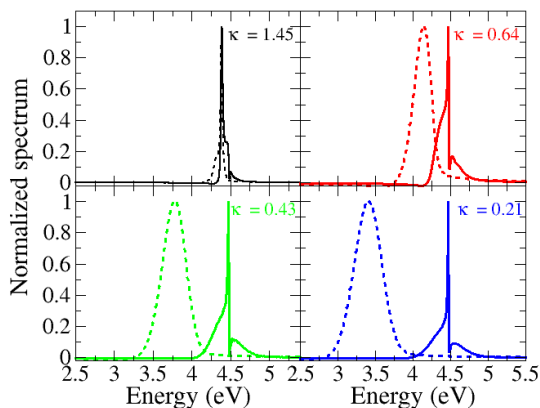
Figure 15 Normalized absorption (solid lines) and emission (dashed lines) spectra for the case with a bright state coupled to a dark state ( H_{12} \neq 0 ) represented in figure 12. The panels correspond to the different spectral densities given in figure 13. \kappa is defined in Eq.(49).
