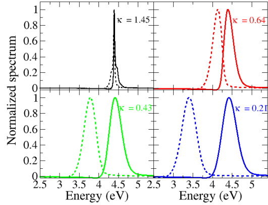
Figure 14 Normalized absorption (solid lines) and emission (dashed lines) spectra for the case with a single bright state ( H_{12} = 0 ) represented in figure 12. The panels correspond to the different spectral densities given in figure 13. \kappa is defined in Eq.(49).
