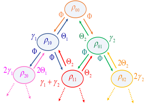
Figure 2 Schematic representation of the auxiliary operators of the HEOM hierarchy up to level L = 2 for the case with two artificial bath modes K = 2 . \Phi acts on matrices for which one occupation number increases by one unit. \Theta_k is applied on matrices for which one occupation number decreases by one unit. The sum of the decay rates n_k \gamma_k multiplying each matrix is indicated. The schematic representation of the terms involved in the derivative of one matrix is complete for \rho_{00} (orange); \rho_{10} (blue) and \rho_{01} (green).
