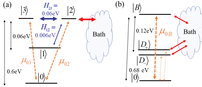
Figure 8 Schematic representation of the energy levels, the interstate couplings H_{ij} , the dipolar couplings \mu_{ij} and the system-bath couplings of a device in which a long-lasting coherence in a dark doublet may be created by interaction with a bath after excitation of a bright state. (a) zero-order basis, (b) eigenstates.
