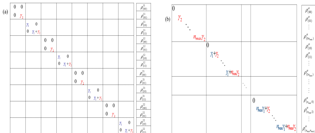
Figure 5 Color on line. Damping superoperator (\mathcal{L}_1 + \mathcal{L}_2)/i (Eqs.(31) and (32)). (a) Example of a two-state system with two artificial decay modes and n_{max} = 1 . \mathcal{L}_1 in blue and \mathcal{L}_2 in red. (b) Block related to a particular element \rho_{ij}^\alpha where \alpha = ij , when n_{max} > 1 . All the blocks (ij) have the same structure
