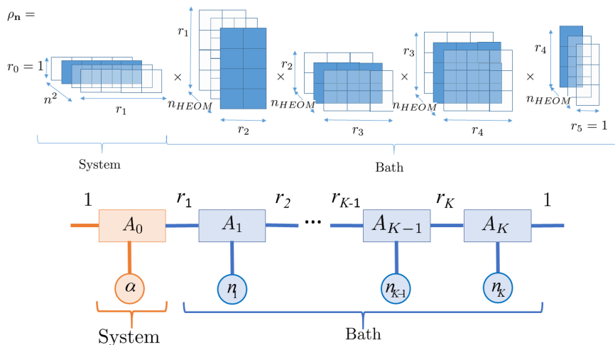
Figure 3 Upper panel : Schematic representation of a tensor train with the HEOM formalism for a two-level system ( n = 2 ) with a bath modelled by two single Tannor-Meier Lorentzian functions with no Matsubara frequencies ( K = 4 ) at a hierarchy level of n_{HEOM} = 3 . Individual matrices or vectors are called cores of the tensor (and often denoted as A_k ). Arbitrary values have been chosen here for the tensor ranks: r_1 = 4 , r_2 = 2 , r_3 = 3 and r_4 = 4 . For instance, the tensor element \rho_{3,2,2,1} , which corresponds to \rho_{3,2,2,1}^{12} , i.e. the element 1,2 of the ADO for occupation number \mathbf{n} = 3, 2, 2, 1 , is computed by performing vector-matrix, matrix-matrix or matrix-vector products with the blue cores on the figure. As the initial and final tensor ranks ( r_0 = r_{K+1} = 1 ) are equal to one, the final result is a scalar number. Lower panel : Tensor train representation of the ADOs. A_k are the cores of the tensor. The circles represent the physical legs. \alpha runs from 1 to n^2 where n is the number of states in the system and n_k is the index (occupation number) for each decay mode that runs from 0 to n_{max} . The rectangles are matrices r_{k-1} \times r_k where the rank r_k is also called the bond.
