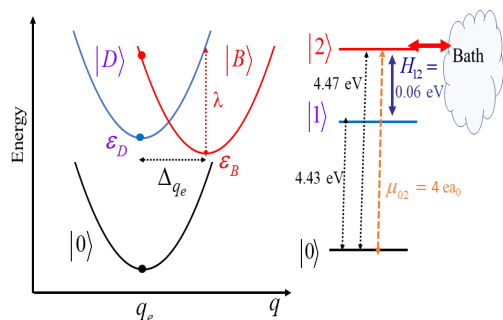
Figure 12 Schematic representation of the diabatic potential energy surface of the excited states used in the simulation of absorption and emission spectra. q is a bath nuclear coordinate and \Delta q_e is the difference of equilibrium positions. The bath is at equilibrium in the ground state and in the dark state |D\rangle since the equilibrium positions are assumed to be the same. The electronic energies of the system correspond to Franck-Condon vertical energies represented by full circles. \lambda is the renormalization energy. Two cases are simulated, the first one with H_{12} = 0 (the |D\rangle state is spectator) and the second one with H_{12} \neq 0
