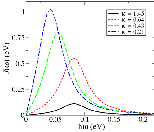
Figure 13 Spectral densities used in the simulation of the absorption and emission spectra. \kappa is defined in Eq.(49). The \Delta parameter is given by the initial value of the correlation function (Eq.(4)). The cutoff \Lambda is estimated by the energy at the maximum. The renormalization energy \lambda for decreasing values of \kappa are 0.034 eV, 0.17 eV, 0.34 eV and 0.52 eV.
