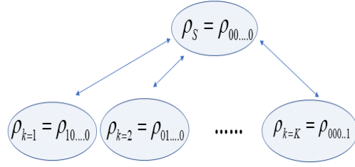
Figure 1 Schematic representation of the auxiliary operators associated to each artificial bath mode k = 1, K and involved in the second order master equation (Eq.(6)). Each ADO corresponds to a single excitation in the mode.
