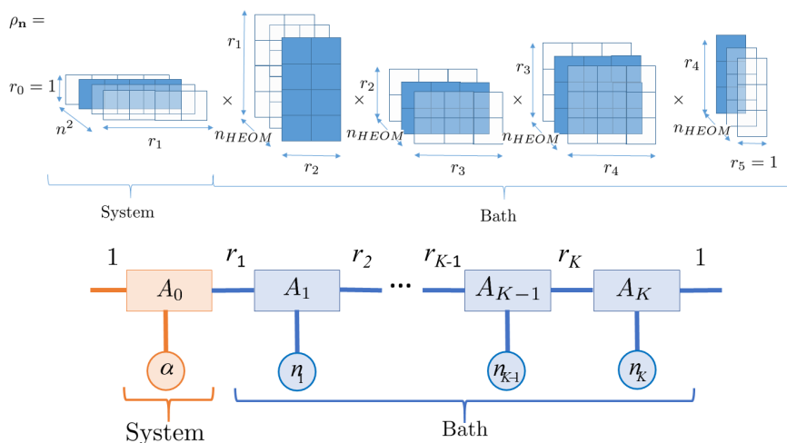
Figure 3 Upper panel : Schematic representation of a tensor train with the HEOM formalism for a two-level system ( n = 2 ) with a bath modelled by two single Tannor-Meier Lorentzian functions with no Matsubara frequencies ( K = 4 ) at a hierarchy level of n_{HEOM} = 3 . Individual matrices or vectors are called cores of the tensor (and often denoted as A_k ). Arbitrary values have been chosen here for the tensor ranks: r_1 = 4 , r_2 = 2 , r_3 = 3 and r_4 = 4 . For instance, the tensor element \rho_{3,2,2,1} , which corresponds to \rho_{3,2,2,1}^{12} , i.e. the element 1,2 of the ADO for occupation number \mathbf{n} = 3, 2, 2, 1 , is computed by performing vector-matrix, matrix-matrix or matrix-vector products with the blue cores on the figure. As the initial and final tensor ranks ( r_0 = r_{K+1} = 1 ) are equal to one, the final result is a scalar number. Lower panel : Tensor train representation of the ADOs. A_k are the cores of the tensor. The circles represent the physical legs. \alpha runs from 1 to n^2 where n is the number of states in the system and n_k is the index (occupation number) for each decay mode that runs from 0 to n_{max} . The rectangles are matrices r_{k-1} \times r_k where the rank r_k is also called the bond.
