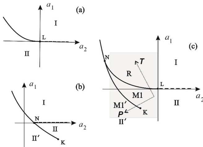
FIG. 12. Equilibrium phase diagram corresponding to free-energy equation (A1) in plane of phenomenological coefficients ( a_1, a_2 ) for (a) canonical six-degree expansion ( a_3 > 0, a_4 = a_5 = 0 ), (b) eight-degree potential ( a_3 < 0, a_4 > 0, a_5 = 0 ), and (c) ten-degree expansion ( a_3 < 0, a_4 < 0, a_5 > 0 ). (c) schematically shows “pressure ( P )-temperature ( T )” plane (gray area, dotted axes). Solid line: first-order; dashed: second-order phase-transition lines. L : Landau tricritical point; N : triple point; K : critical endpoint of isostructural phase transition.
