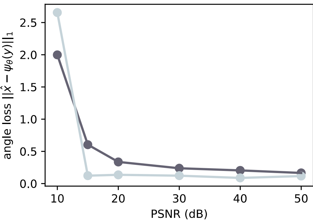
Gaussian noise
