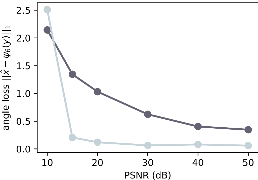
Gaussian noise
