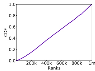
Figure 2: The distribution of domains that trigger EDE codes across the Tranco popularity list.
