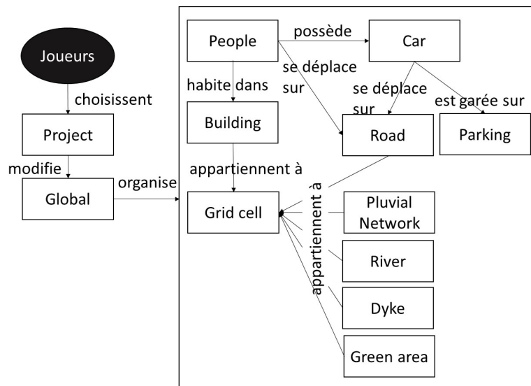
FIGURE 6. Agents de MANA-Flo (Taillandier et al., 2022)
