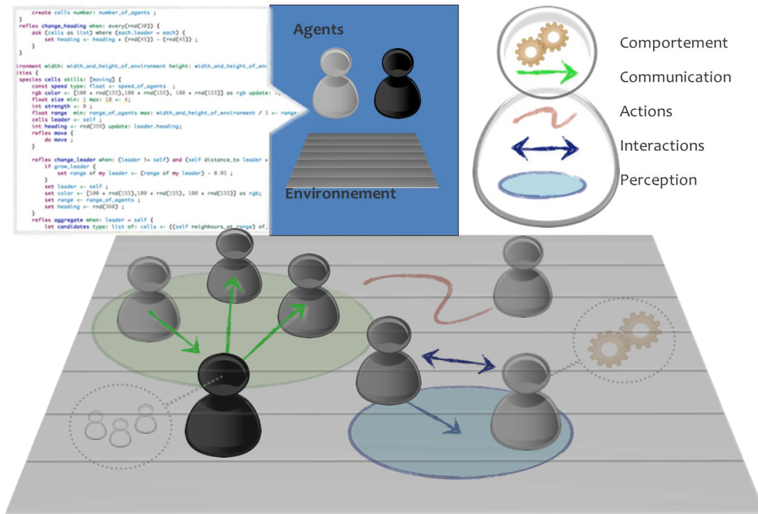
FIGURE 1. Quid ABM ? (Drogoul and Gaudou, 2013)
