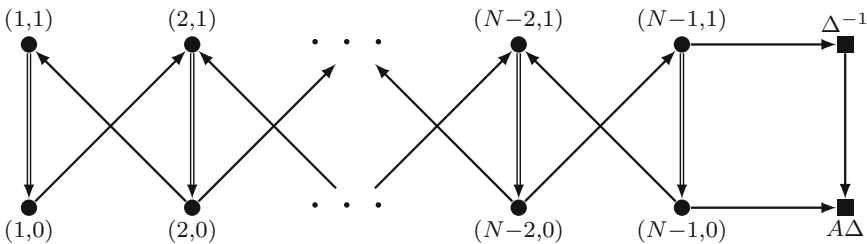
Fig. 2 The type A quantum Q-system quiver corresponding to the initial seed \{Q_{a,0}, Q_{a,1}\} . Square nodes denote coefficients
