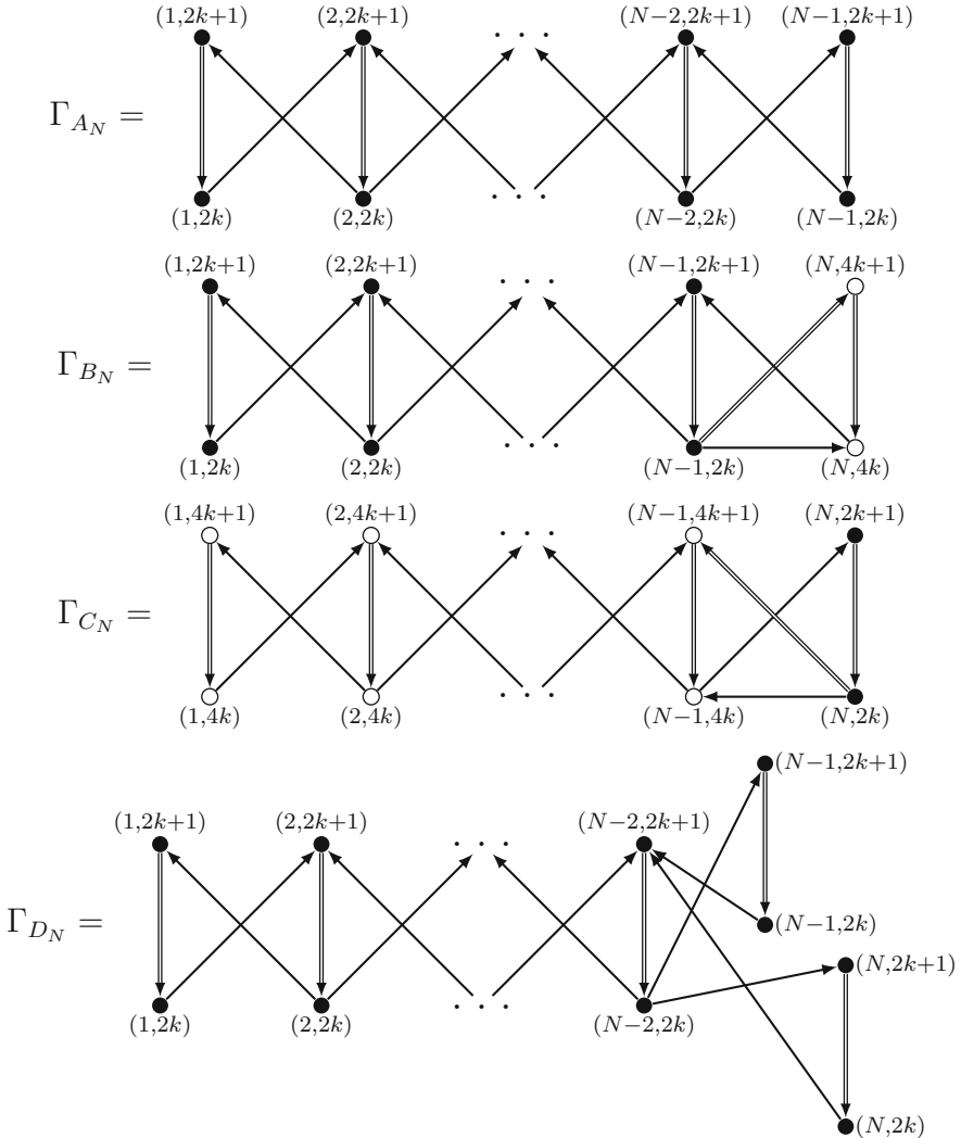
Fig. 1 The quivers for the A_{N-1} , D_N , B_N , C_N Q-system cluster algebras. We have indicated a generic Q-system cluster along the bipartite belt: each vertex labelled (a, k) corresponds to a cluster variable Q_{a,k} . Nodes corresponding to short roots are denoted by empty circles
