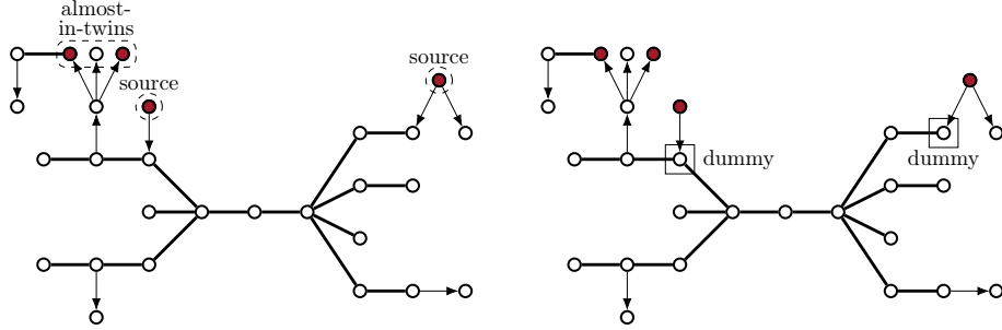
(a) The first step (lines 1-3) is to add every source and manage sets of almost-in-twins.
