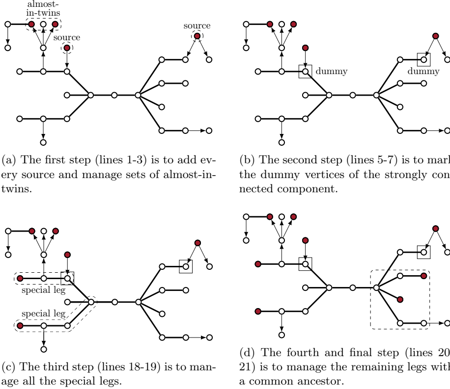
Fig. 1: Illustration of Algorithm 1. For the sake of simplicity, there are only two strongly connected components, for which we only represent the underlying graph with bolded edges, so every bolded edge is a 2-cycle. One of the two strongly connected components is a simple path that does not require any action. Vertices in the metric basis are colored in red.
