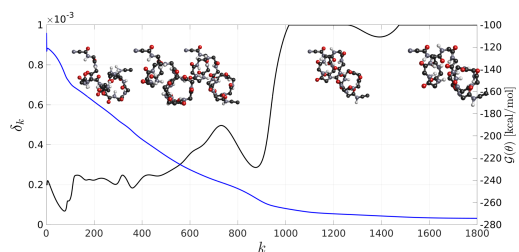
Fig. 2: The free energy of the backbone chain of a protein molecule with a 32-dimensional dihedral angle vector (blue curve; \mathcal{G}(\theta) on the right axis), its transient conformations, and the step-size of the explicit \Psi TC scheme (black curve; \delta_k on the left axis). The five plotted backbone chain conformations from left to right correspond to iterations 100, 300, 500, 1000, and 1400, respectively.
