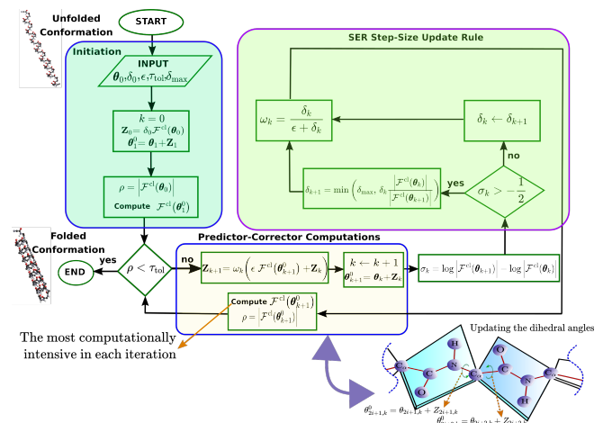
Fig. 1: The flow chart of the proposed explicit \Psi TC scheme for integrating the KCM-based forward dynamics of protein molecules modeled as hyper-redundant serial robotic mechanisms.
