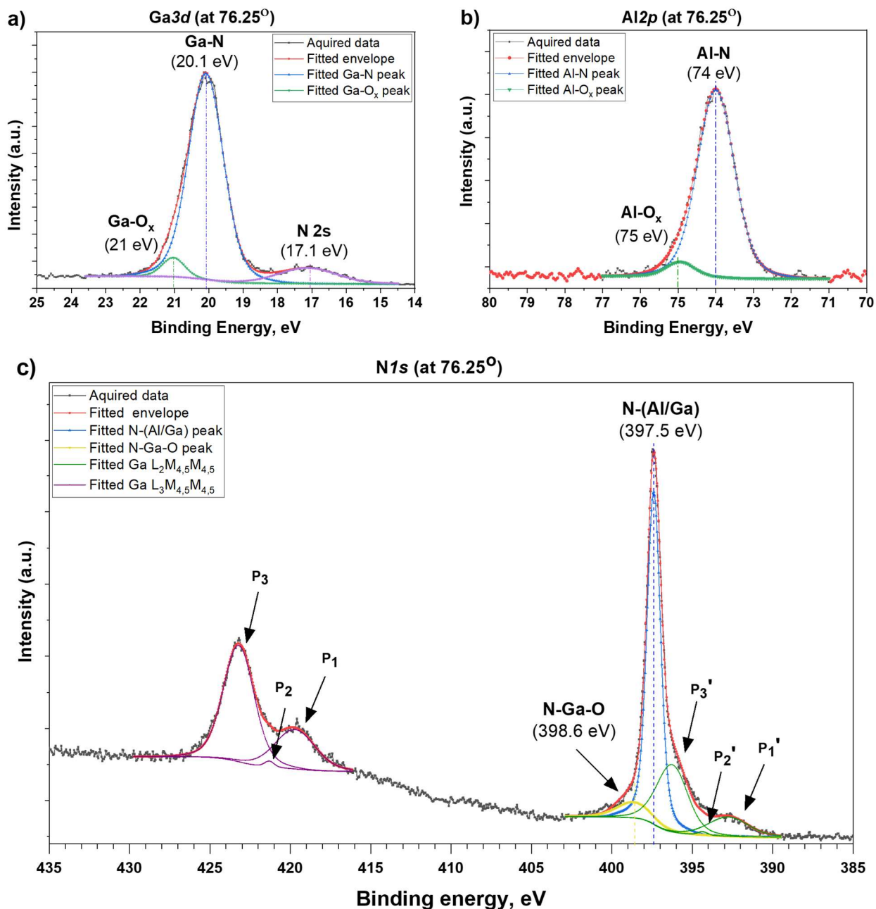
Fig. 4. (a) Ga3d , (b) Al2p , and (c) N1s core levels deconvolution of AR-XPS spectra of the reference AlGa N sample measured at 76.25^\circ .
