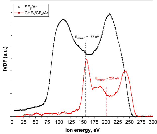
Fig. 2. Measured average ion velocity distribution function (IVDF) during high-energy SF 6 /Ar plasma (black line) and high-energy CHF 3 /CF 4 /Ar plasma etching processes.
