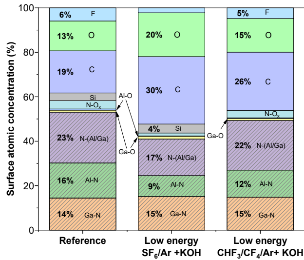
Fig. 13. The atomic composition of the AlGa N sample at grazing angle 76.25° (surface) for reference sample and samples after etching by low-energy SF 6 /Ar and CHF 3 /CF 4 /Ar followed by KOH
