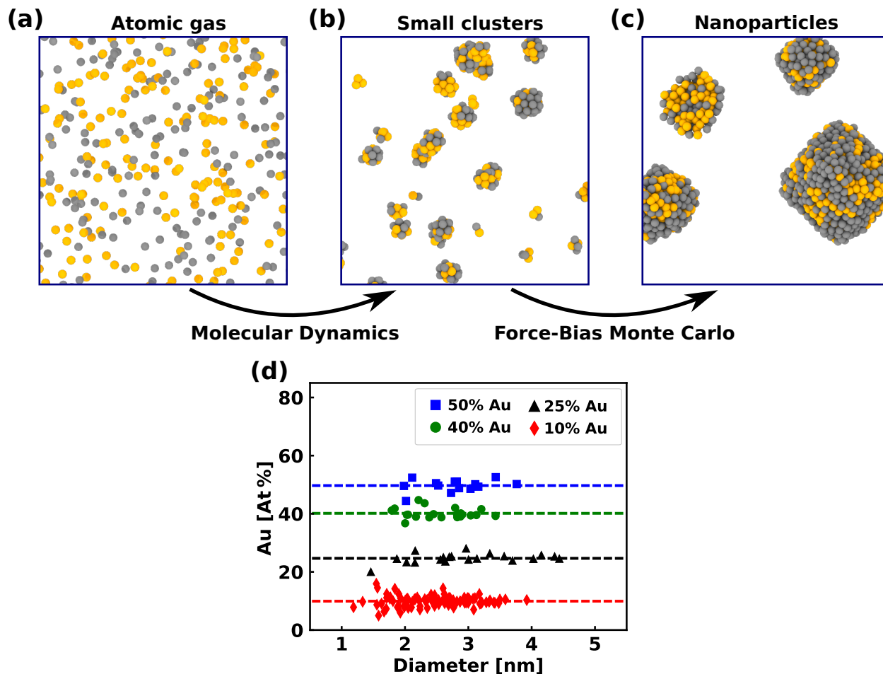
Figure 5: Hybrid MD/FBMC approach to study Au-Ag nanoparticle aggregation. (a) An initial atomic Au/Ag gas evolves to (b) a set of small clusters using MD. Then, FBMC is implemented to mimic a longer-timescale process of (c) nanometer-sized particle growth. For the sake of simplicity, in (a)-(c), we just show a piece of the whole simulation box. The chemical composition of individual nanoparticles is given by points with shapes indicated by the legend. The average composition (with their corresponding standard deviation) of each are 50 \pm 2\% (for 50% in Au), 40 \pm 2\% (for 40% in Au), 25 \pm 2\% (for 25% in Au) and 10 \pm 2\% (for 10% in Au).
