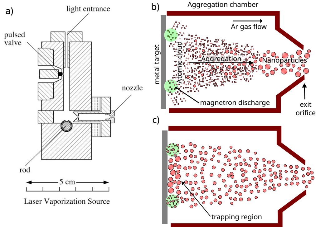
Figure 1: a) Scheme of a laser vaporization source. A laser pulse hits a rod target, eroding it and producing a localized plasma of \sim 1 \text{ mm}^3 for a very short time. The plasma is quenched by a pulse of inert gas that condensates the metal vapor into nanoparticles. (b-c) Schematic of a magnetron sputtering cluster source with its round metal target, usually 1 or 2 inches in diameter. The magnetron discharge forms a torus and erodes the target, producing the metal vapor that is used to form the nanoparticles. (b) The standard picture of nanoparticle formation starts from the atomic metal vapor, followed by the nucleation, successive atom addition, and finally, cluster coalescence all the way between the discharge and the exit orifice of the aggregation chamber, usually a few hundred millimeters long. (c) Recent works by Kousal et al. 25,26 propose that the nanoparticles are formed very close to the sputter target and not all along the aggregation chamber. Also, they demonstrate that trapping regions exist in the center of the plasma torus, where the biggest nanoparticles are trapped.
