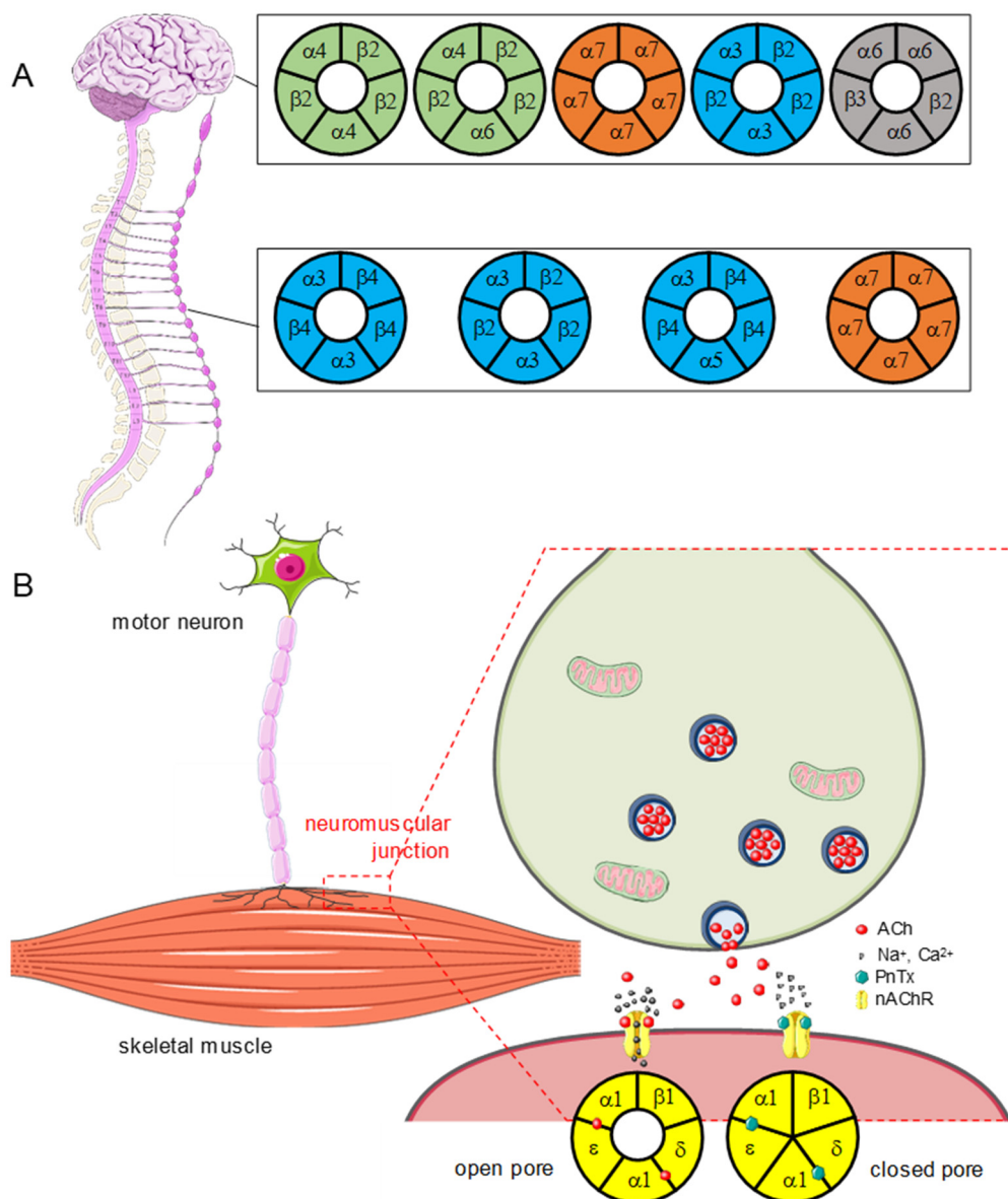
Figure 2. PnTXs act as competitive antagonists of nicotinic acetylcholine receptors (nAChRs). (A) Central (upper) and peripheral (lower) nAChRs, as a function of their subunit composition. Some nAChRs are exclusively present in the CNS or in the PNS, for instance the ganglia of the autonomous system. Others, like \alpha_7 homopentamers or \alpha_3\beta_2 heteropentamers, are expressed in both. Note that only a few of the existing nAChRs are represented ( \alpha_7\beta_2 , \alpha_4\beta_2 for example are not presented, see [19,20]). (B) Mode of action of PnTXs at the neuromuscular junction. The toxins bind to the sites where it normally binds on the nAChR expressed at the surface of the endplate muscle membrane, thus impairing the opening of the cationic pore. When the receptor is inhibited, it cannot promote the depolarization of the endplate membrane, which impairs the generation of a muscle action potential and thereby the initiation of muscle contraction.
