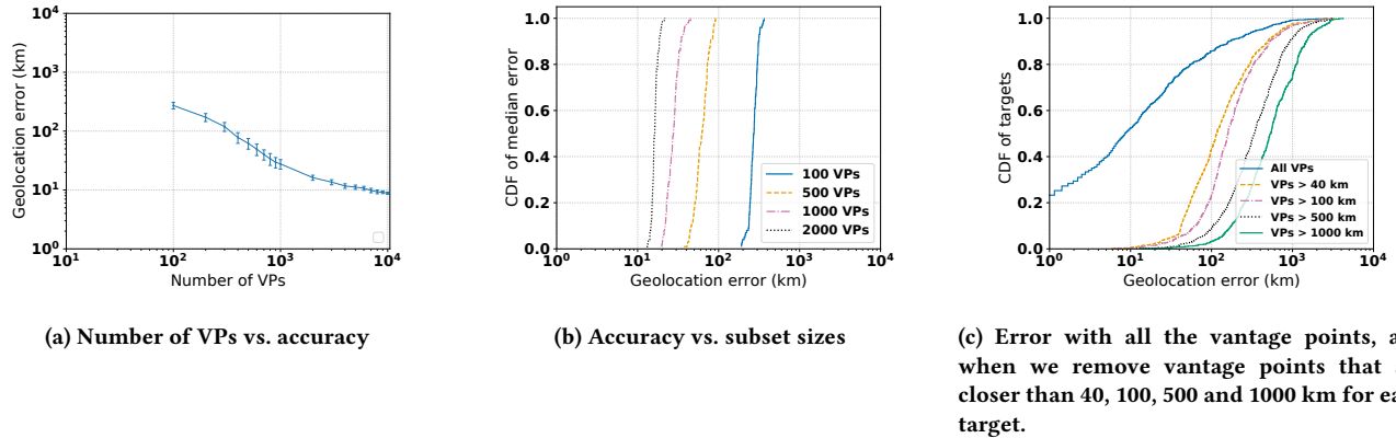
Figure 2: Replication of the three hypotheses on how using subsets of VPs affect accuracy.
