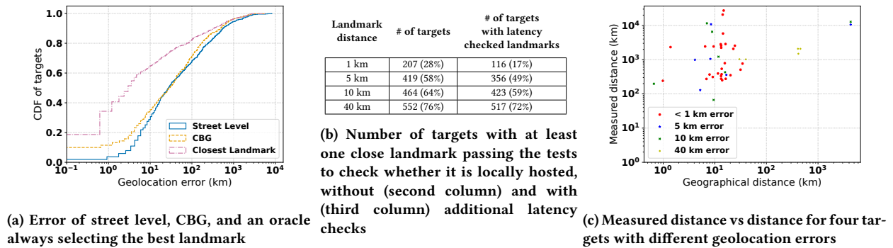
Figure 5: Performance of the street level technique (left) and re-evaluation of the two insights: is there a close landmark for most targets (middle)? Is the relative order of the geographical distance preserved by the measured distance (right)?
