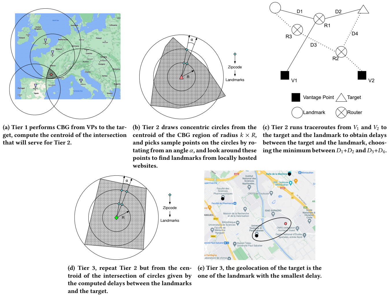
Figure 1: Three tier technique to geolocate an IP address in the street level paper [46]
