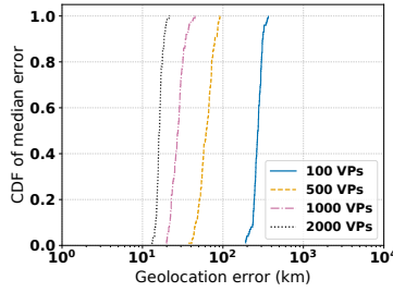
(b) Accuracy vs. subset sizes
