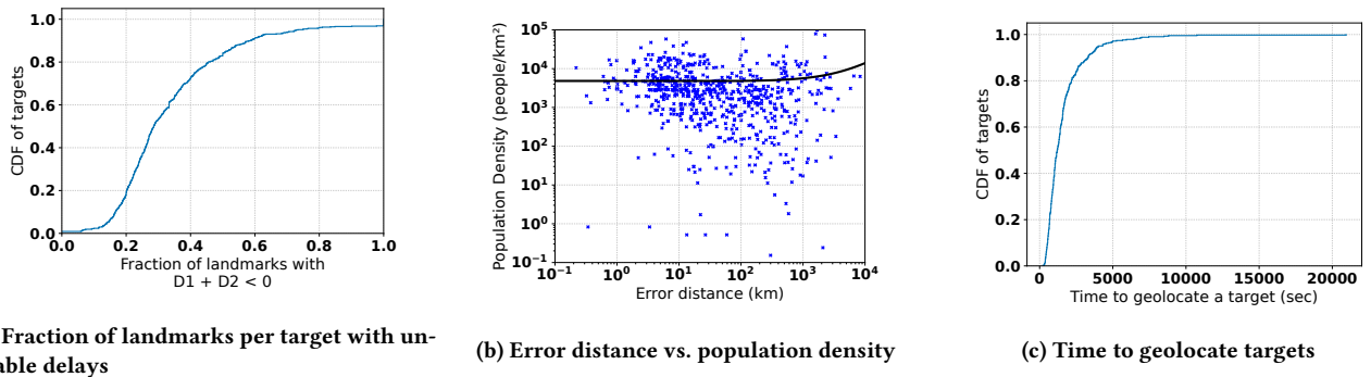
Figure 6: Delays between landmark and targets are noisy (left), accuracy does not depend on the population density (middle), the technique hardly scales with our setup (right).
