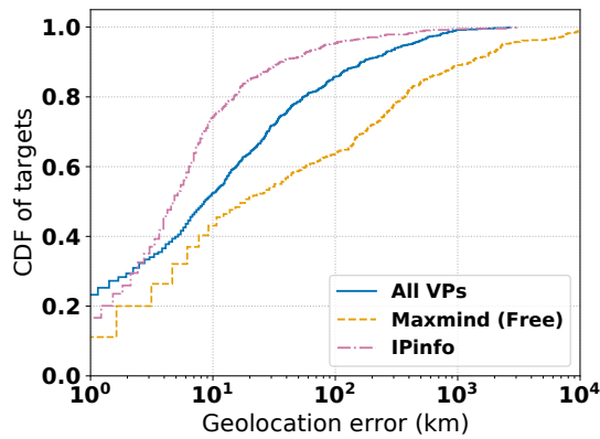
Figure 7: Geolocation of CBG with all the RIPE Atlas VPs versus geolocation databases.
