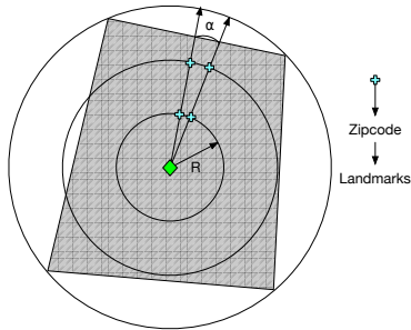
(d) Tier 3, repeat Tier 2 but from the centroid of the intersection of circles given by the computed delays between the landmarks and the target.
