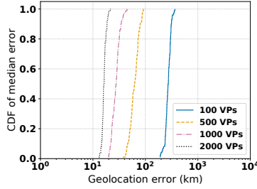
(b) Accuracy vs. subset sizes
