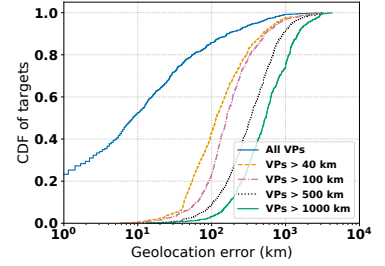
(c) Error with all the vantage points, and when we remove vantage points that are closer than 40, 100, 500 and 1000 km for each target.
