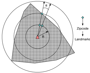
(b) Tier 2 draws concentric circles from the centroid of the CBG region of radius k \times R , and picks sample points on the circles by rotating from an angle \alpha , and look around these points to find landmarks from locally hosted websites.
