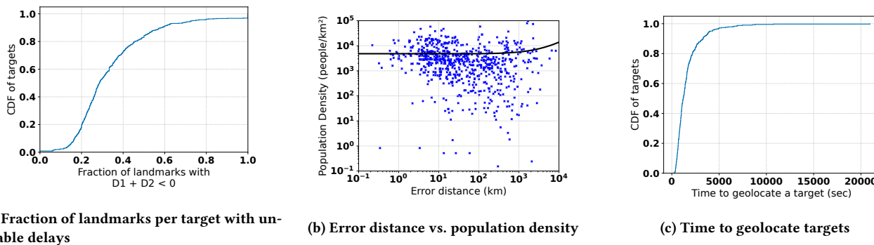
Figure 6: Delays between landmark and targets are noisy (left), accuracy does not depend on the population density (middle), the technique hardly scales with our setup (right).
