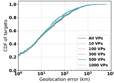
(b) Error when using two steps VP selection algorithm to reduce measurement overhead, with different sizes of subsets of VPs for the first step.
