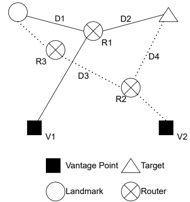
(c) Tier 2 runs traceroutes from V_1 and V_2 to the target and the landmark to obtain delays between the target and the landmark, choosing the minimum between D_1 + D_2 and D_3 + D_4 .
