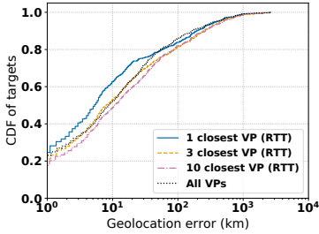
(a) Error when using VPs with the lowest RTTs to IP addresses within the same prefix as the target (original VP selection algorithm) vs using all VPs.
