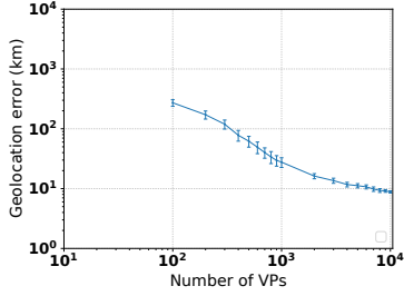
(a) Number of VPs vs. accuracy
