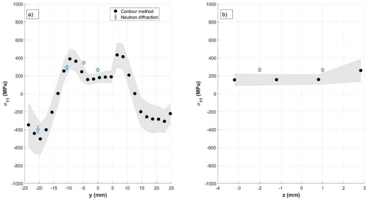
Figure 14: Comparison of neutron diffraction and contour method on the longitudinal residual stress along a) y -axis and b) z -axis. Grey surface corresponds to the combined standard uncertainty taking into account the dispersion of the results over the surface on which the average stress was calculated, and the uncertainty related to the contour method, estimated at 50 MPa
