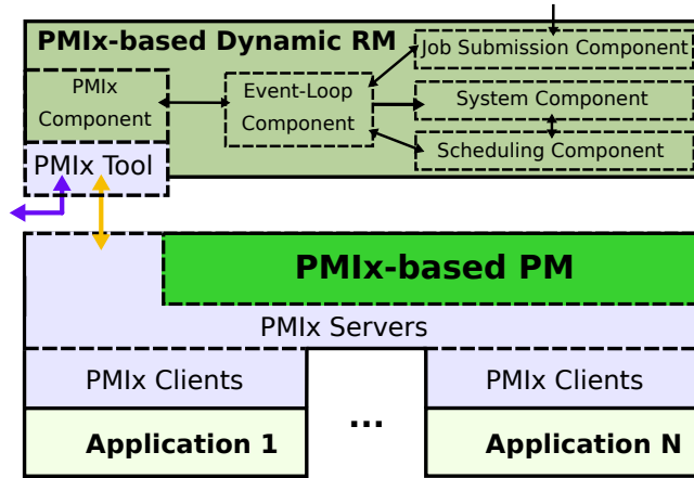
Fig. 1: Overview of an architecture for PMIx-based interactions between the Resource Manager (RM) and the Process Manager (PM). The bottom part represents the PM, which manages the execution of one or more applications. It operates PMIx servers to expose certain services to the application processes or other software components via the PMIx Client and PMIx Tool interface. The top part represents a RM manager consisting of various components. The PMIx component is responsible for managing the PMIx-based connection and interaction with the PM (yellow arrow) and possibly other system components (blue arrow) using the PMIx Tool interface. Note, that although the PM could potentially manage multiple applications across multiple nodes, the RM only needs to connect to one of the PM’s PMIx servers, which facilitates the scalability of the approach.
