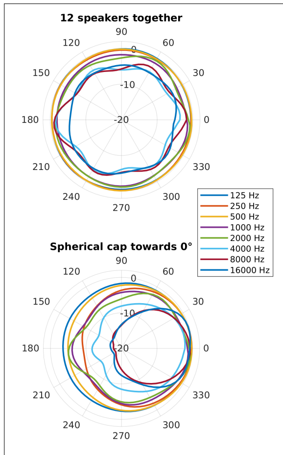
Figure 2. Directivity patterns normalized by the maximum value in the horizontal plane of the controlled source. Top: 12 drivers playing together. Bottom: Only one driver playing to the front, i.e. spherical cap condition.
