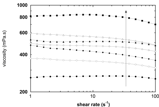
Fig. 6 shear-rate dependence of the viscosity of the double emulsion as a function of the PVPone concentration in oil. The initial oil fraction is kept constant at 0.5. The arrow indicates the increase of the concentration of PVPone, from 0 to 20 wt. %.
