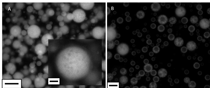
Fig. 8 Dark field microscopy images of double emulsions prepared with PNIPAM-COOH co-dispersed with PEG in 1-octanol, at A) high pH and B) after decreasing the pH. The scale bar is 20 \mu\text{m} for both images, and 5 \mu\text{m} for the inset figure A.
