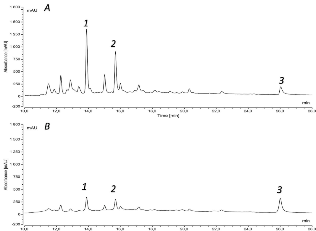
Fig. 2. Chromatograms of TAN A after water (A) or methanol (B) extraction obtained by HPLC-DAD at 250 nm. Peak identification 1: gallic acid, 2: vescalagin, 3: ellagic acid.
