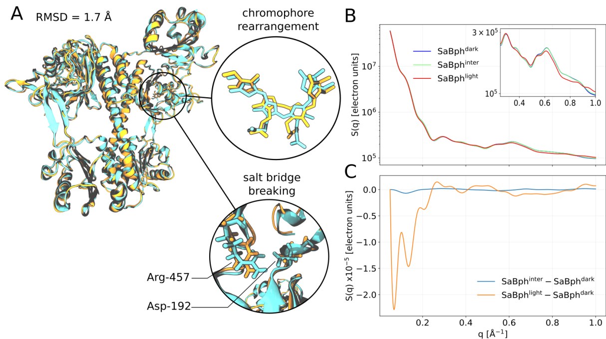
Figure 2 - Effect of protein conformational changes on difference scattering patterns. (A) The structure of bacteriophytochrome from Stigmatella aurantiaca (SaBph) in the dark form (SaBph dark , PDB 6PTQ, cyan cartoon and licorice representation) and in a 5 ns photo-activated form (SaBph light , PDB 7JR5, orange cartoon and licorice representation) are superimposed for comparison. After 5 ns from photoexcitation the chromophore structure is significantly different from the ground state one; moreover, the relative distance of several helices has changed and a functionally relevant salt bridge is broken [14]. The root mean-square deviation (RMSD) for the two structures is 1.7 Å. (B and C) For illustrative purposes, we artificially divided the overall conformational change in an initial step in which only the chromophore rearrangement has occurred (we call this artificial state SaBph inter ) and a second step in which also the polypeptide conformational change is present (SaBph light ). The absolute scattering patterns corresponding to these three states have been calculated using the WAXSiS webserver [15] and are reported in panel B , the inset representing an enlarged view of the high scattering angles region. While the three absolute patterns have the same overall shape, they differ in small details that are directly linked to the structural changes represented in panel A . This is better highlighted by plotting the difference between two scattering patterns, which is typically referred to as the TR-XSS signal. (C) Comparison of the SaBph inter -SaBph dark scattering difference (blue) with the SaBph 5ns -SaBph dark scattering difference (orange). The panel highlights that an overall (although small) protein structural change results in a much larger TR-XSS signal than a structural change localized on the chromophore.
