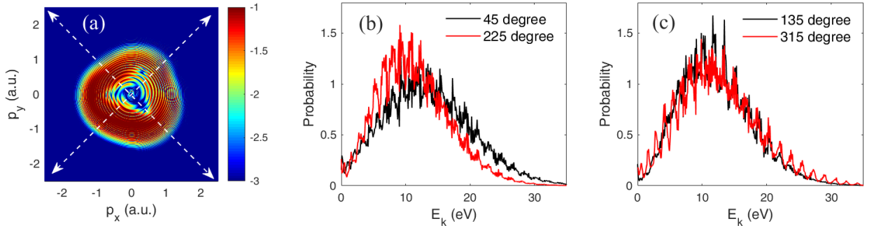
Fig. 5. (a) The photoelectron momentum spectrum without the DC electric field. In (b) and (c), the photoelectron kinetic energy distributions are presented. In (b), the black line denotes that the DC electric field points to 45 degree and the red line refers to an opposite direction (225 degree) to the black one. In (c), the black (red) line corresponds to electric field at 135° and 315°. The calculating parameters: E_{800} = 2.5 \times 10^{14} W/cm 2 , E_{400} = 5 \times 10^{12} W/cm 2 , \tau = 40 fs, E_{DC} = 3 kV/cm and effective DC electric field duration of 4.8 ps before plasma screening.
