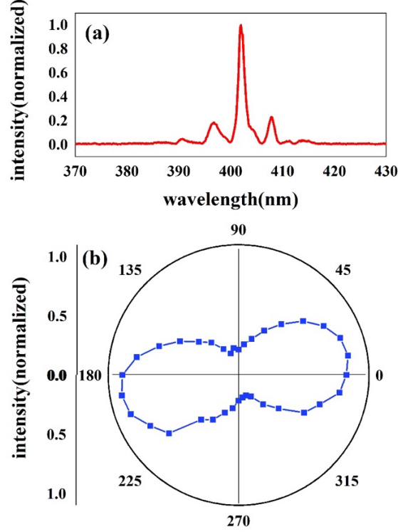
Figure 4. Measured spectrum (a) and polarization (b) of the parasitic second harmonic generated on the quarter wave-plate.
