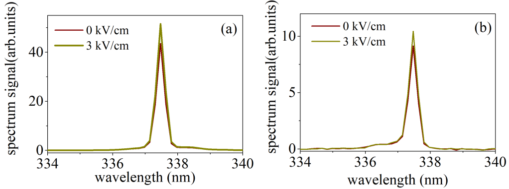
Fig. 2. The influence of the applied electric field on the 337.4 nm signal measured 1 meter away from the plasma. (a) and (b) respectively show the forward and backward 337.4 nm spectral signals for different strengths of electric field. The spectra were averaged over about 3000 laser shots.
